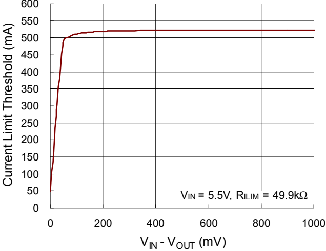
Current Limit Threshold vs. ( V_{IN} - V_{OUT} )
