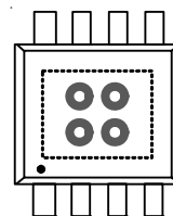
Figure 4. Standard PTH to GND Plane
