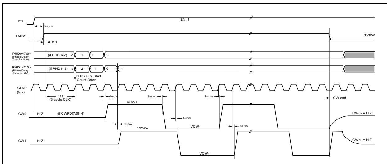
FIGURE 4-4: CW0~7 Output Timing Diagram.
