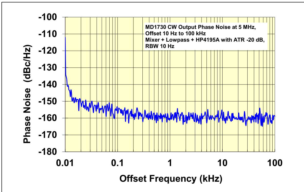
FIGURE 2-13: Typical CW Output Phase Noise Curves.
