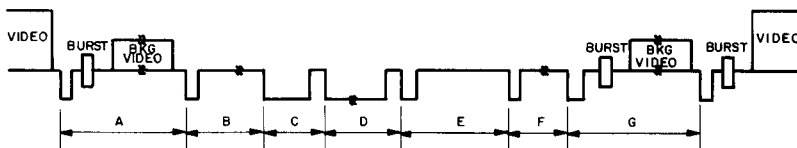
Fig. 8 - Vertical sync timing (see Table 7).
