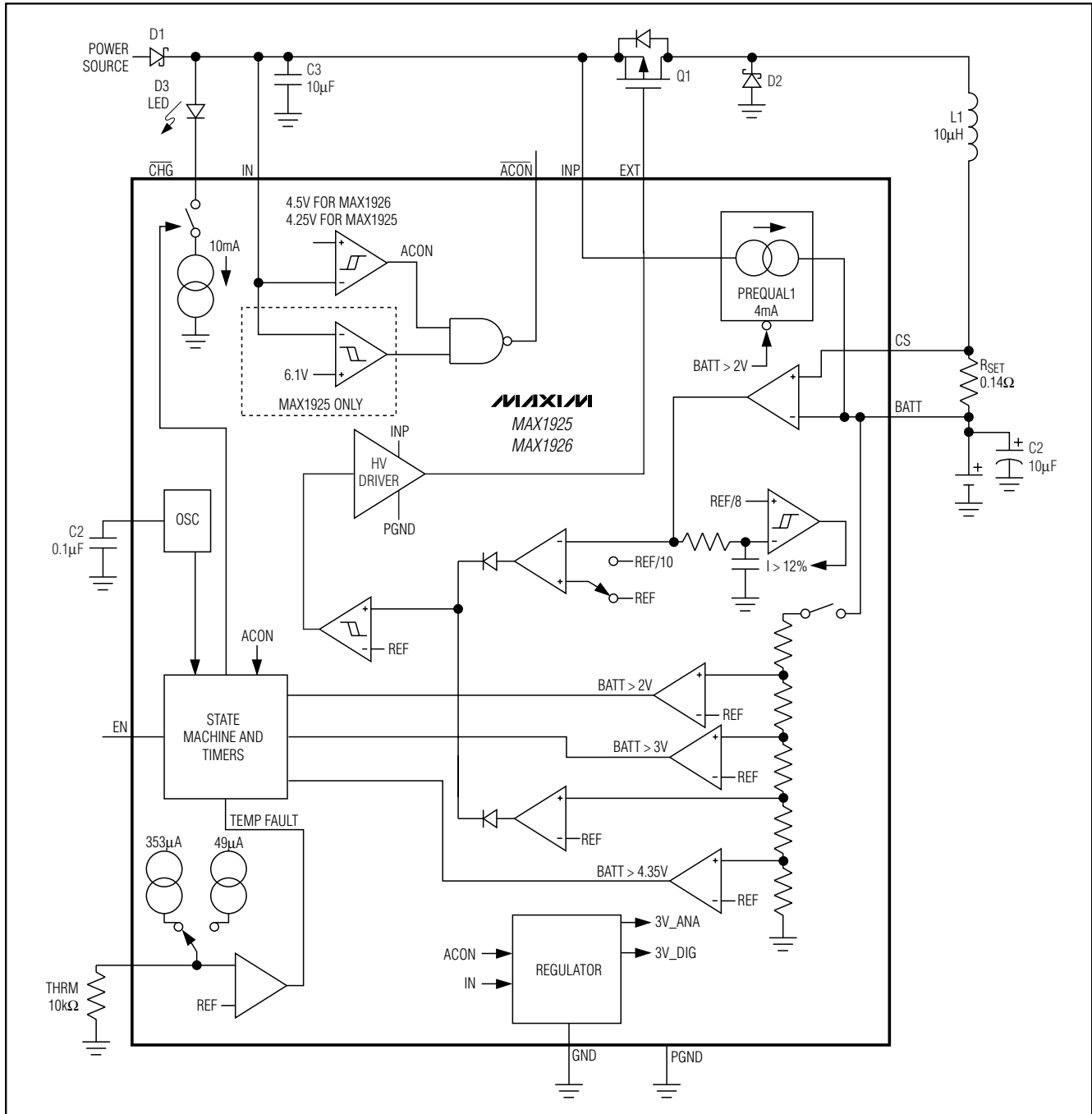
Figure 1. Functional Diagram
