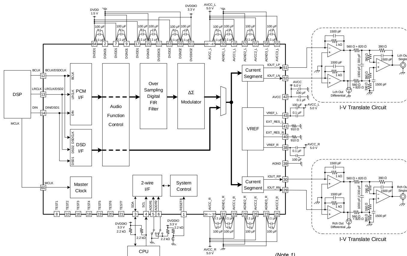
Figure 37. Application Circuit
