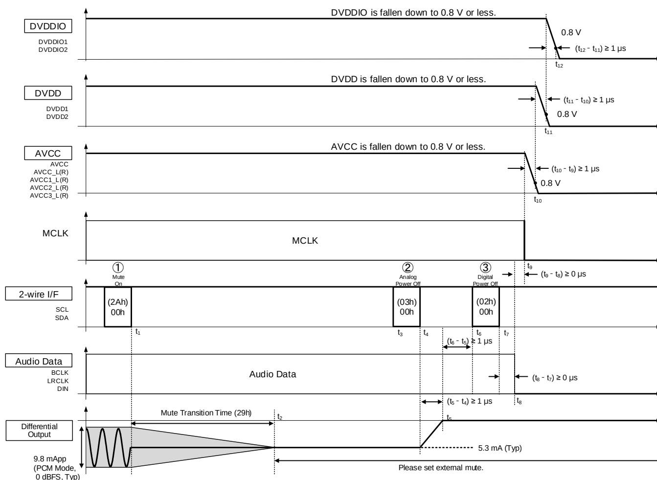
Figure 33. Power-Off Sequence
