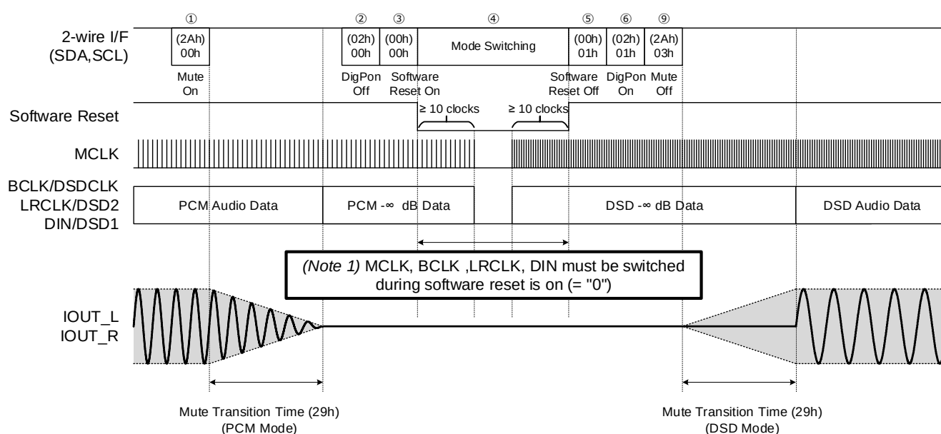
Figure 34. Mode Switching Sequence from PCM Mode to DSD Mode
