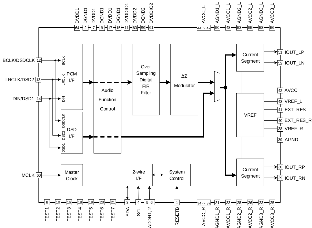
Figure 3. Block Diagram
