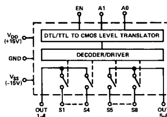
AD7502
