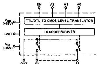
AD7502
