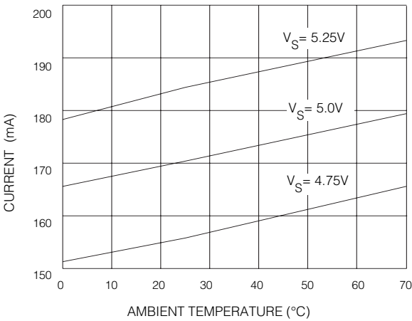
Fig. 15 Supply Current
