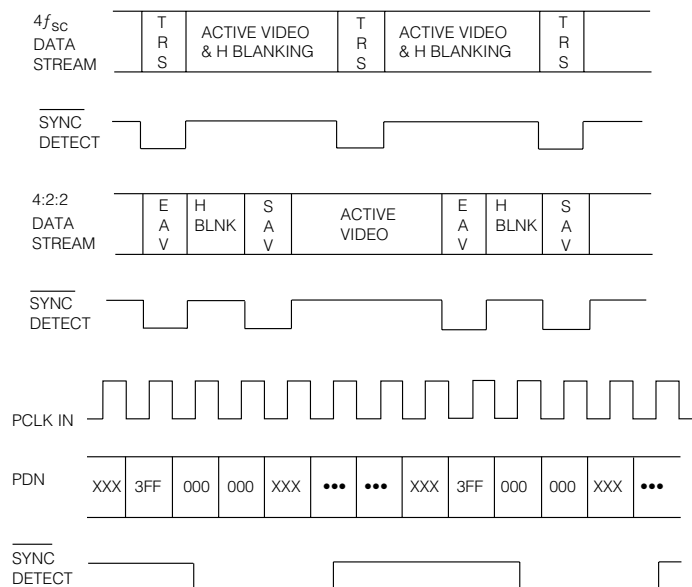
Fig. 10 Timing Diagram
