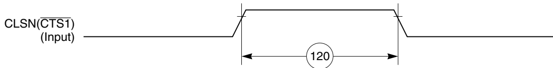
Figure 57. Ethernet Collision Timing Diagram
