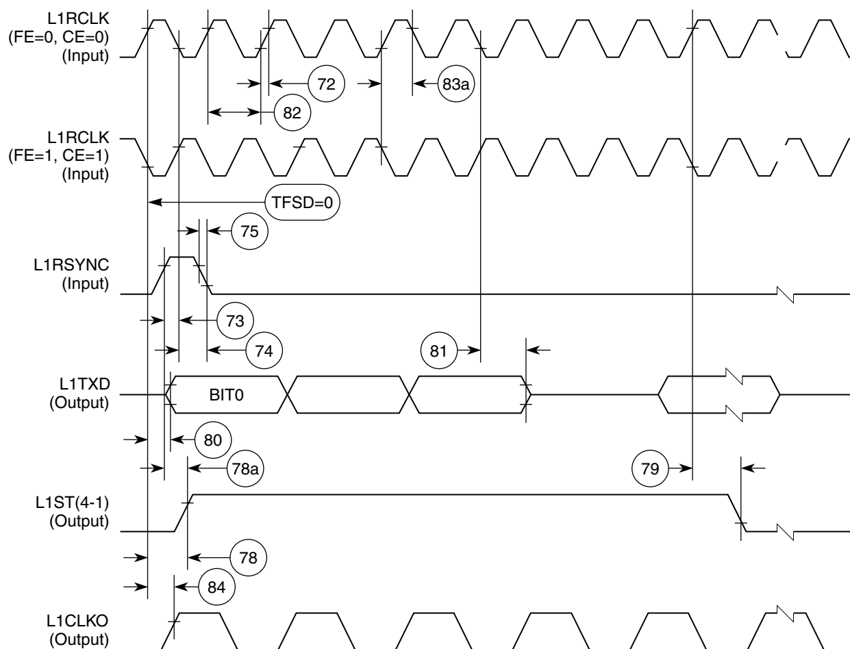
Figure 52. SI Transmit Timing with Double Speed Clocking (DSC = 1)
