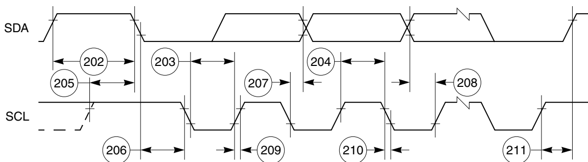
Figure 67. I 2 C Bus Timing Diagram
