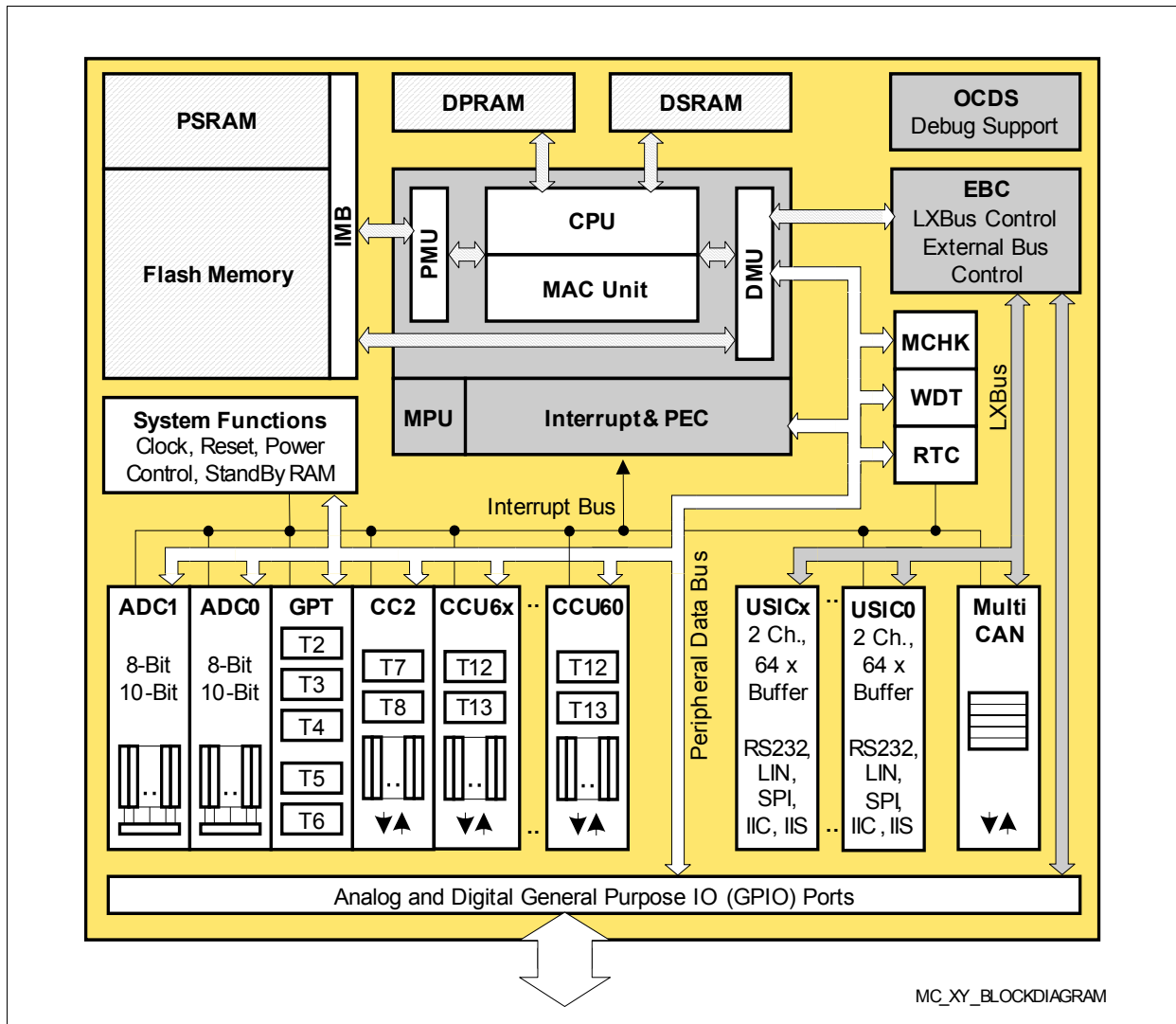
Figure 3 Block Diagram
