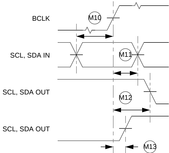
Figure 9. I2C and System Clock Timing Relationship
