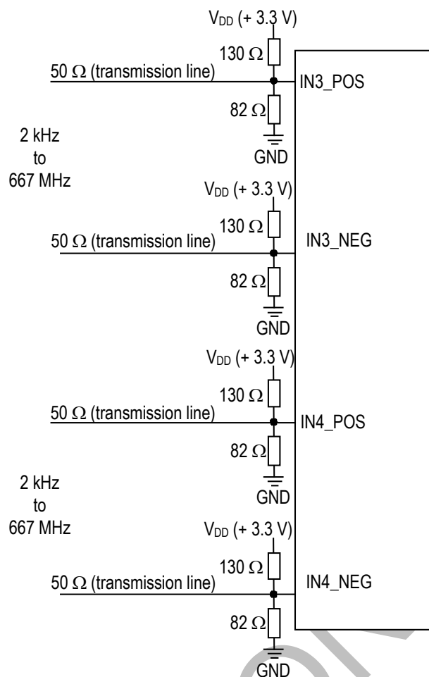
Figure 30. Recommended PECL Input Port Line Termination
