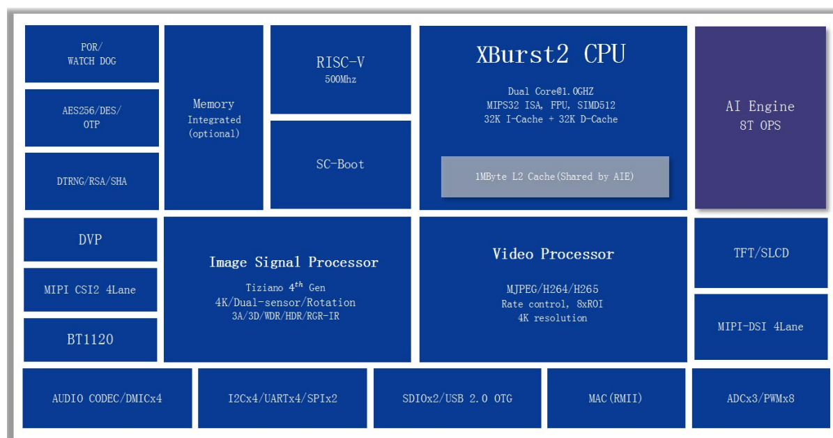
Figure 1-1 T40N Diagram
