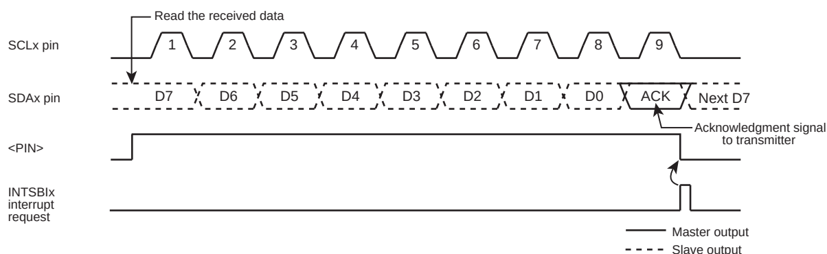
Figure 11-11 <BC[2:0]>= "000", <ACK>= "1" (Receiver Mode)
