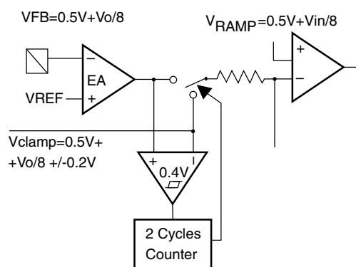
Figure 6. Duty-Cycle Clamp
