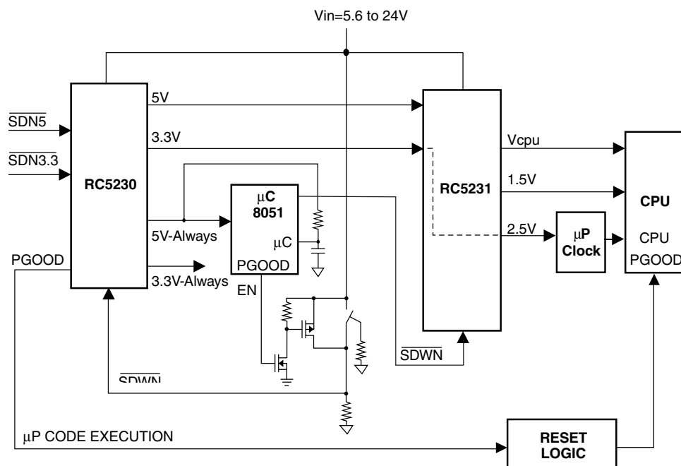
Figure 7. System Block Diagram
