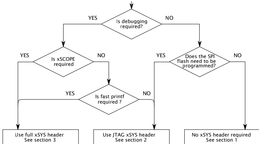
Figure 32: Decision diagram for the xSYS header
