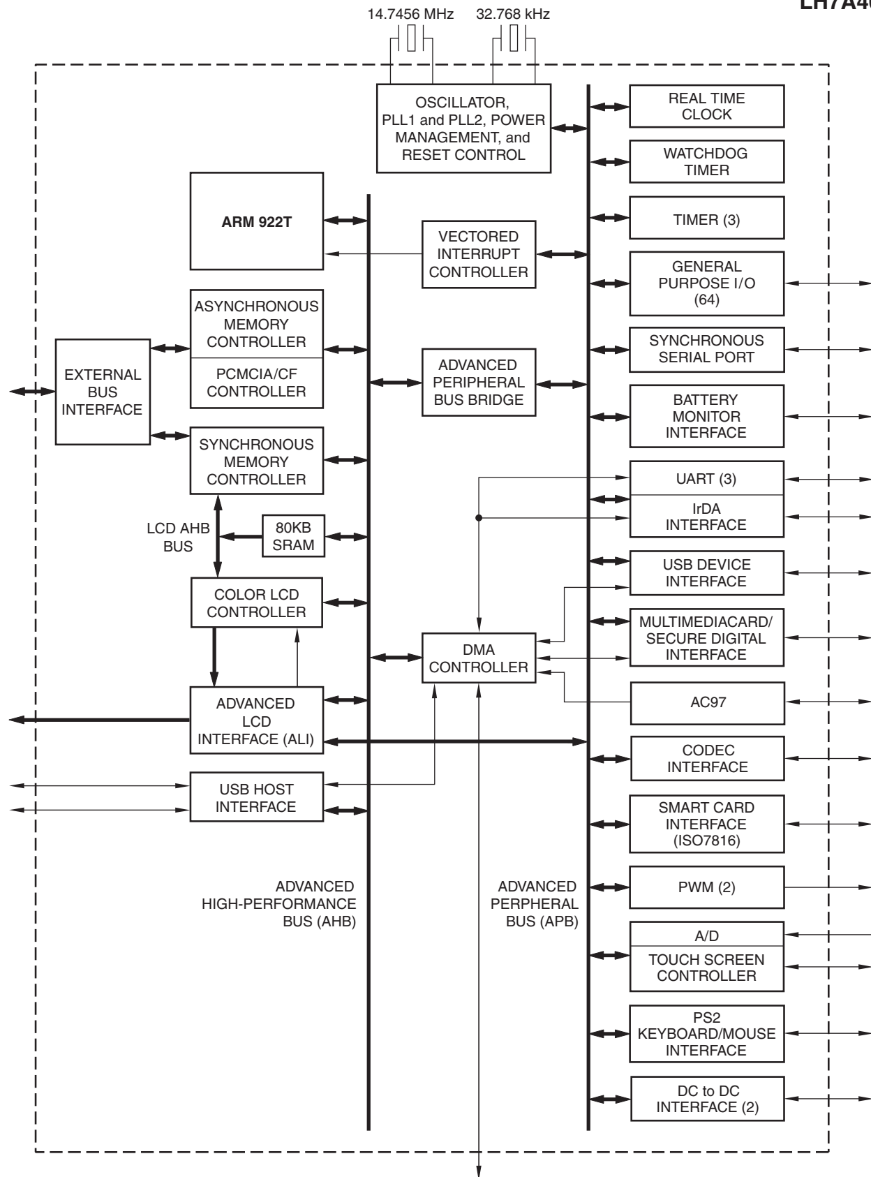
Figure 1. LH7A404 Block Diagram
