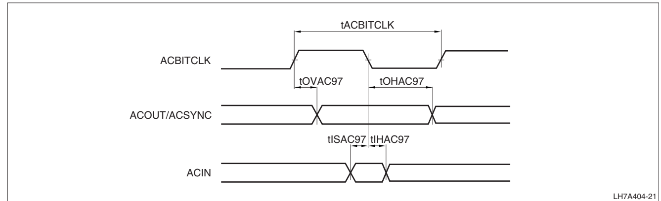
Figure 30. AC97 Data Setup and Hold
