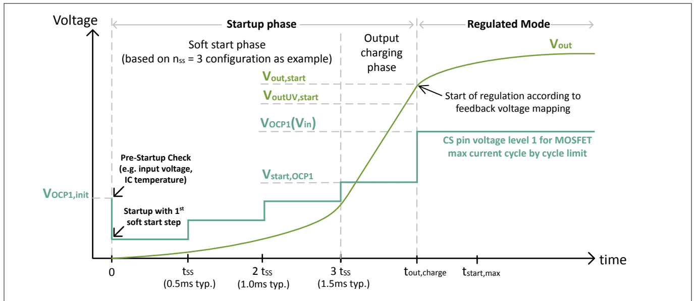
Figure 12 Startup phase with soft start step n_{\text{ss}}=3
