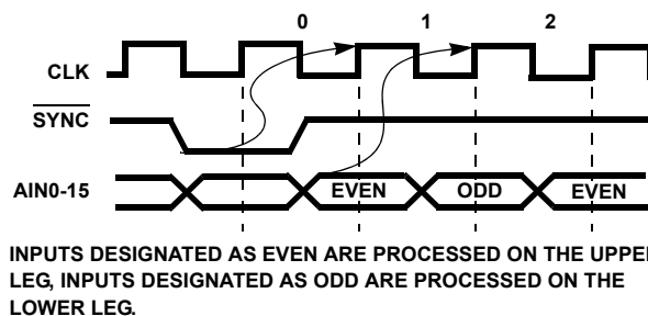
FIGURE 8. DATA SYNCHRONIZATION WITH PROCESSING LEGS ( \overline{\text{INT/EXT}} = 1 )
