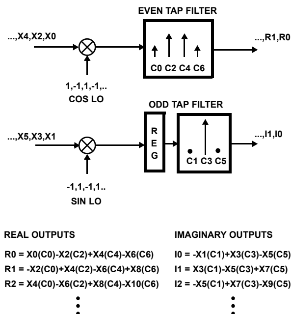
FIGURE 14. DOWN CONVERT AND DECIMATE FUNCTION USING POLYPHASE FILTERS
