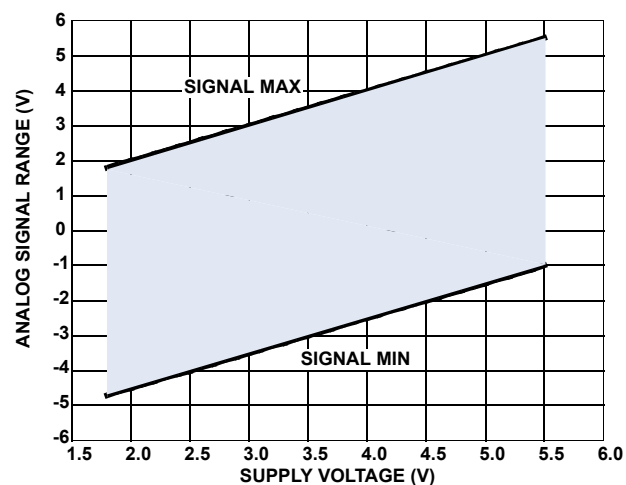
FIGURE 14. ANALOG SIGNAL RANGE vs SUPPLY VOLTAGE
