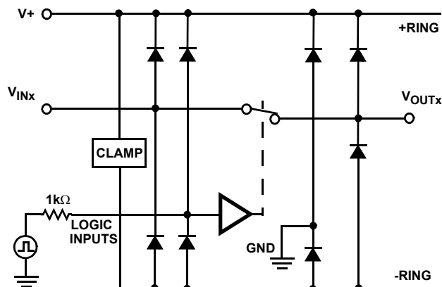
FIGURE 8. OVERVOLTAGE PROTECTION
