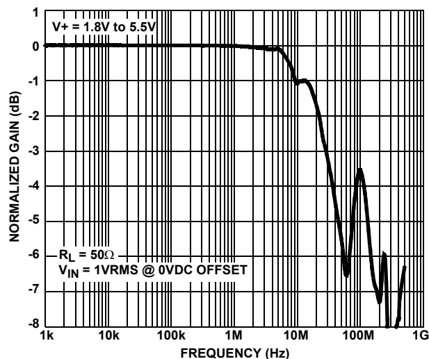
FIGURE 19. FREQUENCY RESPONSE
