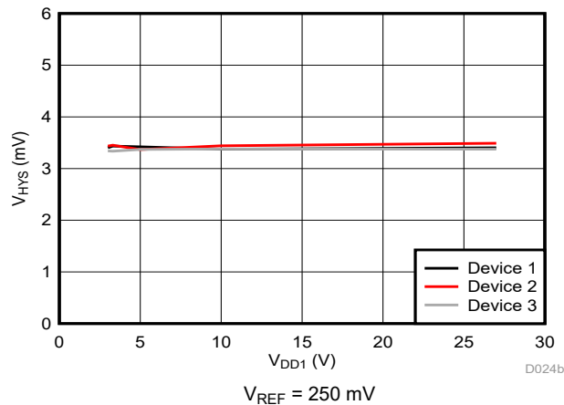
Figure 6-15. Cmp0 Trip Threshold Hysteresis vs Supply Voltage
