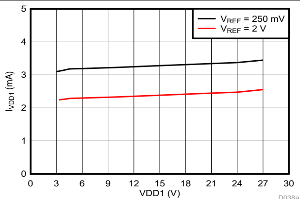
Figure 6-43. High-Side Supply Current vs Supply Voltage
