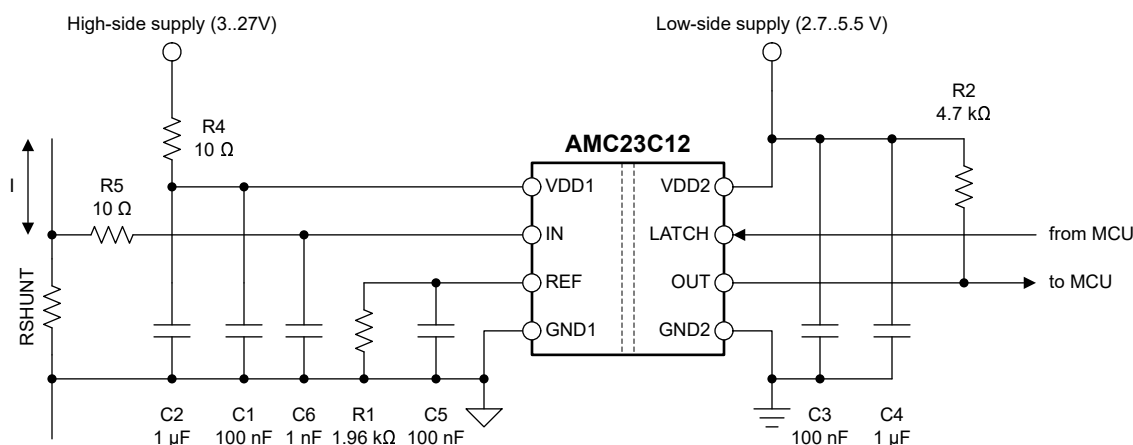
Figure 8-6. Decoupling of the AMC23C12
