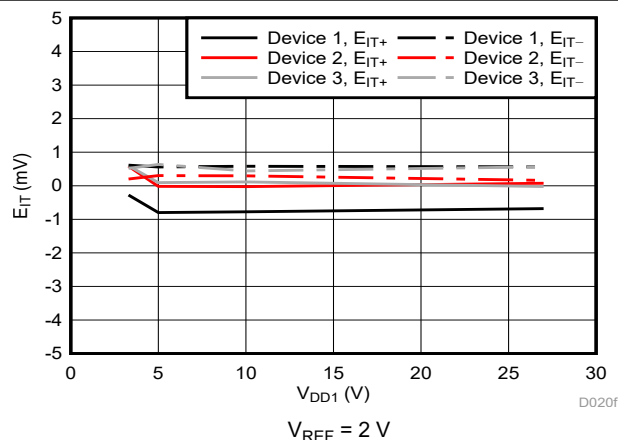
Figure 6-19. Cmp0 Trip Threshold Error vs Supply Voltage
