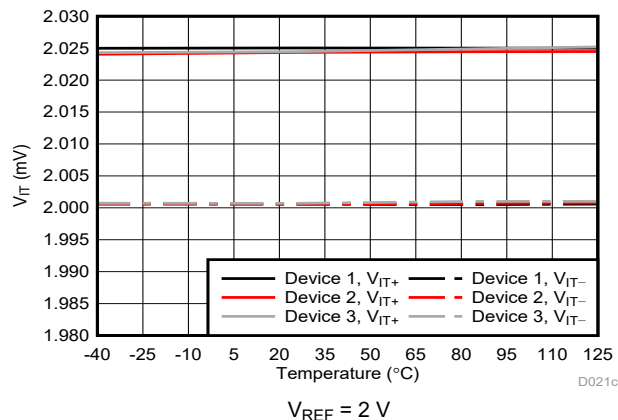
Figure 6-18. Cmp0 Trip Threshold vs Temperature
