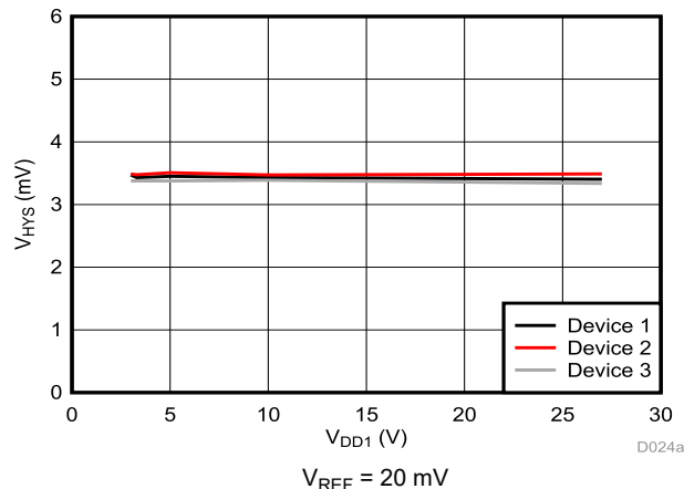
Figure 6-9. Cmp0 Trip Threshold Hysteresis vs Supply Voltage
