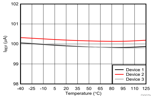
Figure 6-42. Reference Current vs Temperature
