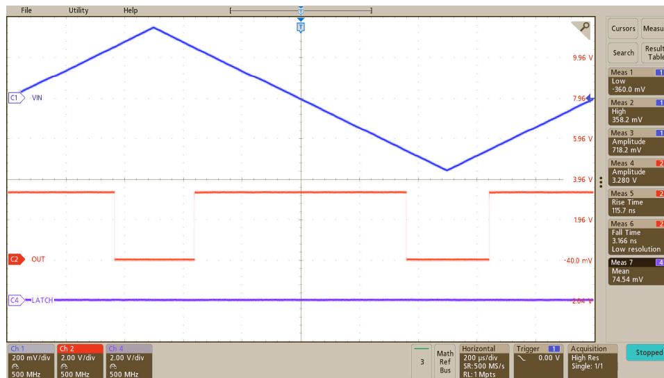
Figure 8-3. Output Response of the AMC23C12 to a Triangular Input Waveform
