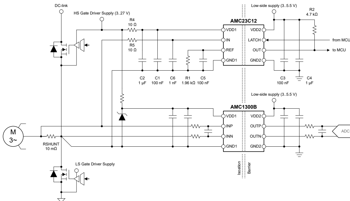
Figure 8-1. Using the AMC23C12 for Overcurrent Detection
