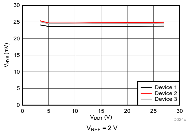
Figure 6-21. Cmp0 Trip Threshold Hysteresis vs Supply Voltage
