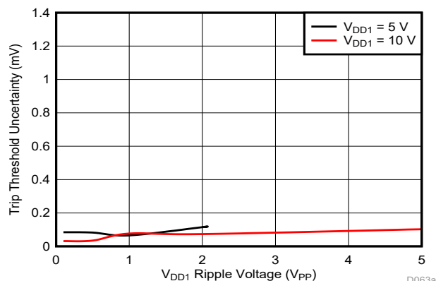
Figure 8-4. Trip Threshold Sensitivity to VDD1 Ripple Voltage (Cmp0, f_{\text{RIPPLE}} = 10 \text{ kHz} )
