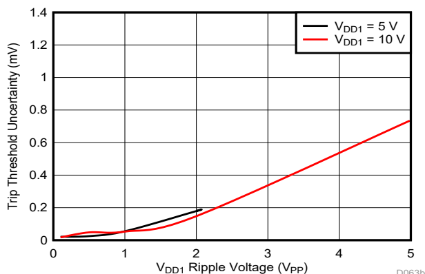
Figure 8-5. Trip Threshold Sensitivity to VDD1 Ripple Voltage (Cmp1, f_{\text{RIPPLE}} = 10 \text{ kHz} )
