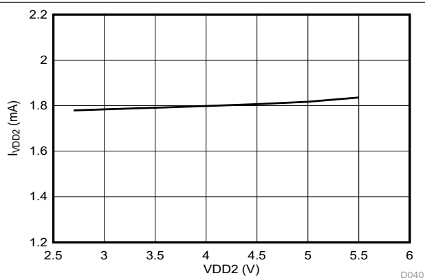
Figure 6-43. High-Side Supply Current vs Supply Voltage
