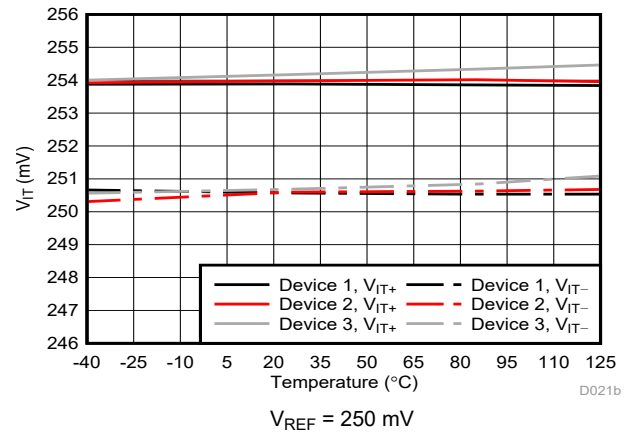
Figure 6-12. Cmp0 Trip Threshold vs Temperature
