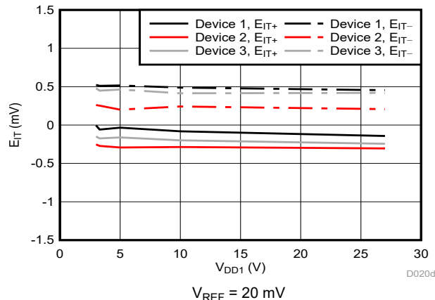
Figure 6-7. Cmp0 Trip Threshold Error vs Supply Voltage
