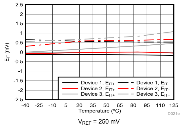
Figure 6-14. Cmp0 Trip Threshold Error vs Temperature
