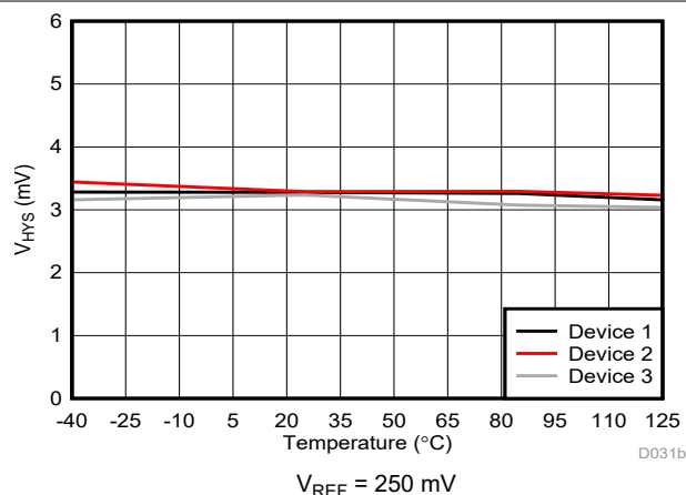
Figure 6-34. Cmp1 Trip Threshold Hysteresis vs Temperature
