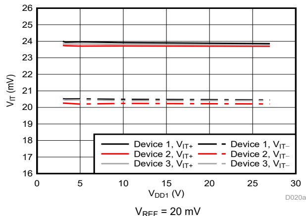
Figure 6-5. Cmp0 Trip Threshold vs Supply Voltage
