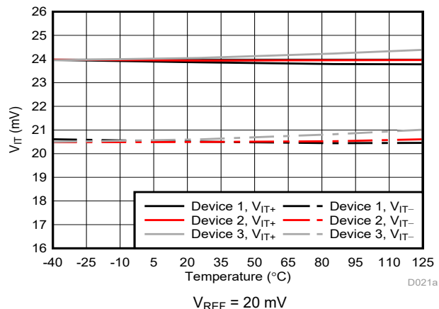
Figure 6-6. Cmp0 Trip Threshold vs Temperature
