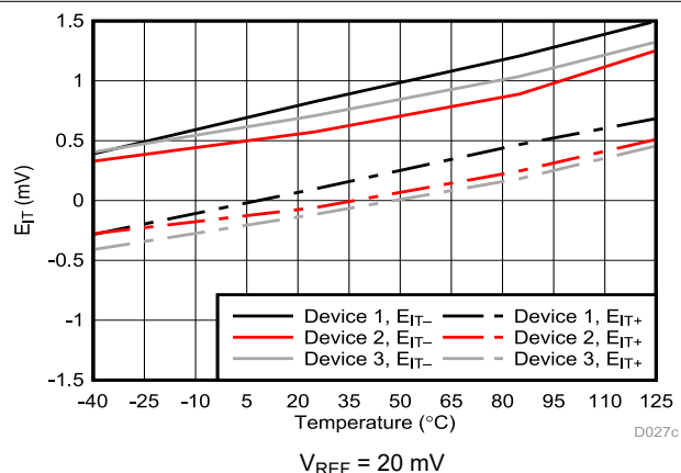
Figure 6-26. Cmp1 Trip Threshold Error vs Temperature
