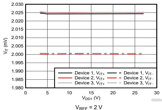
Figure 6-17. Cmp0 Trip Threshold vs Supply Voltage
