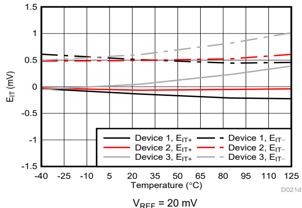
Figure 6-8. Cmp0 Trip Threshold Error vs Temperature
