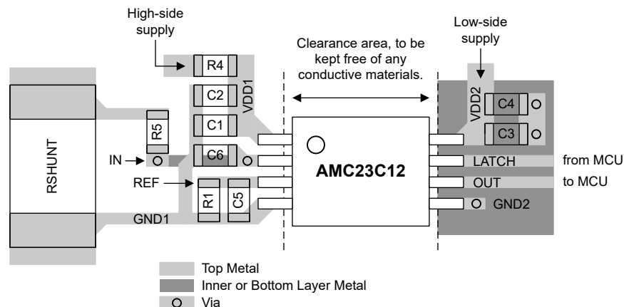
Figure 8-7. Recommended Layout of the AMC23C12
