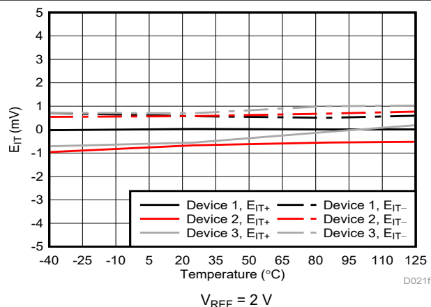
Figure 6-20. Cmp0 Trip Threshold Error vs Temperature
