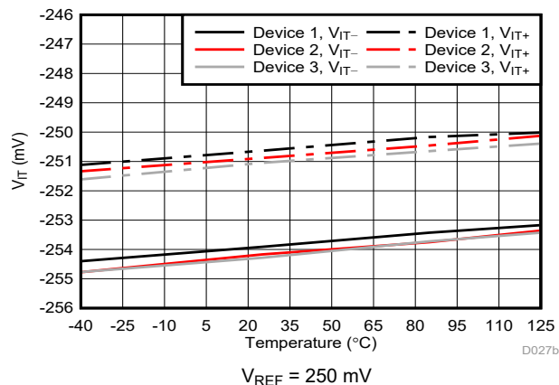
Figure 6-30. Cmp1 Trip Threshold vs Temperature
