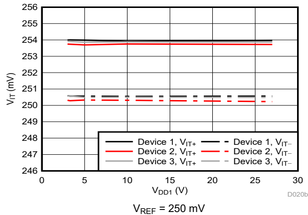
Figure 6-11. Cmp0 Trip Threshold vs Supply Voltage
