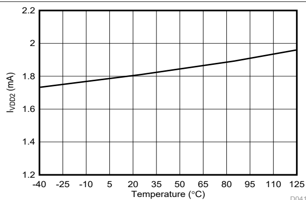
Figure 6-44. High-Side Supply Current vs Temperature
