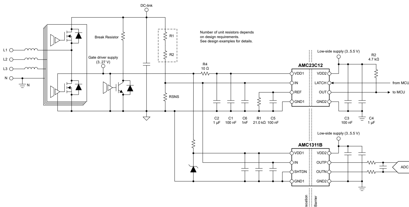
Figure 8-2. Using the AMC23C12 for Overvoltage Detection
