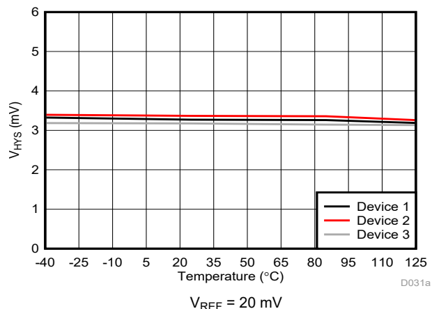
Figure 6-28. Cmp1 Trip Threshold Hysteresis vs Temperature
