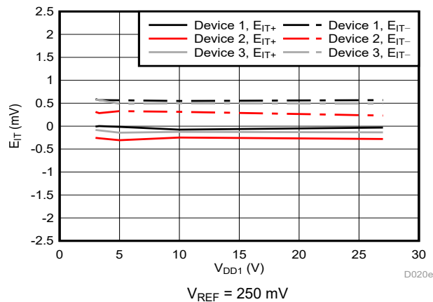
Figure 6-13. Cmp0 Trip Threshold Error vs Supply Voltage
