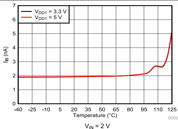
Figure 6-40. Input Bias Current vs Temperature
