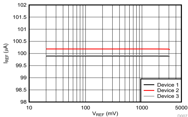
Figure 6-41. Reference Current vs Reference Voltage
