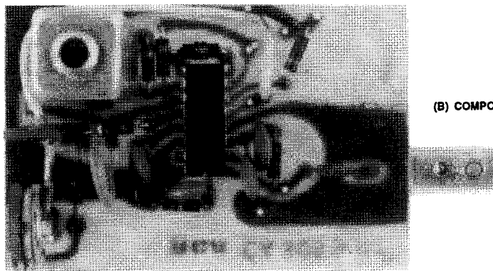
FIGURE 5. ACTUAL SIZE PHOTOGRAPHS OF THE CA3089E &amp; OUTBOARD COMPONENTS MOUNTED ON A PRINTED-CIRCUIT BOARD.
