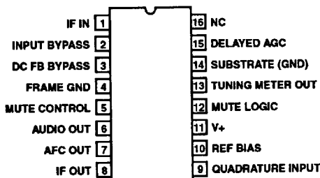
CA3089 (PDIP, CDIP) TOP VIEW
