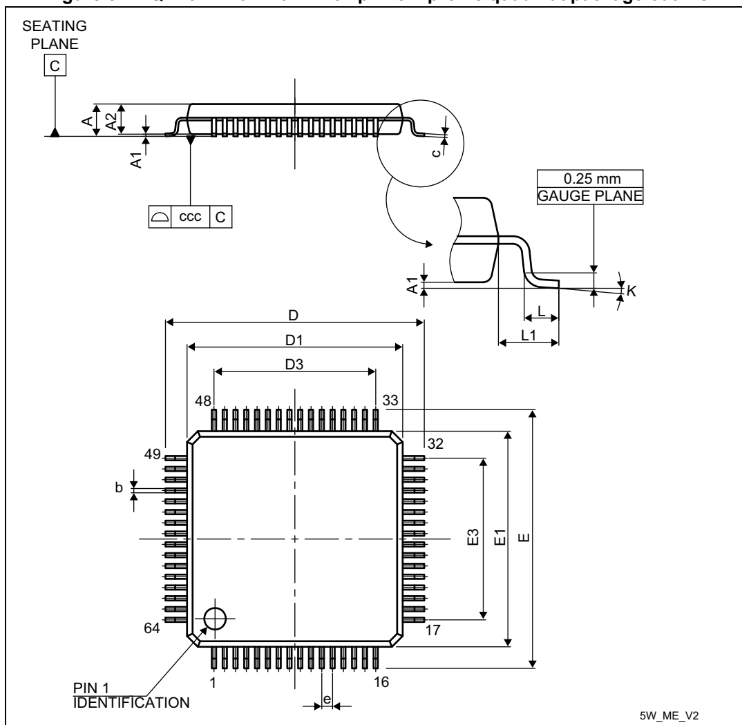
Figure 34. LQFP64 – 10 x 10 mm 64 pin low-profile quad flat package outline
