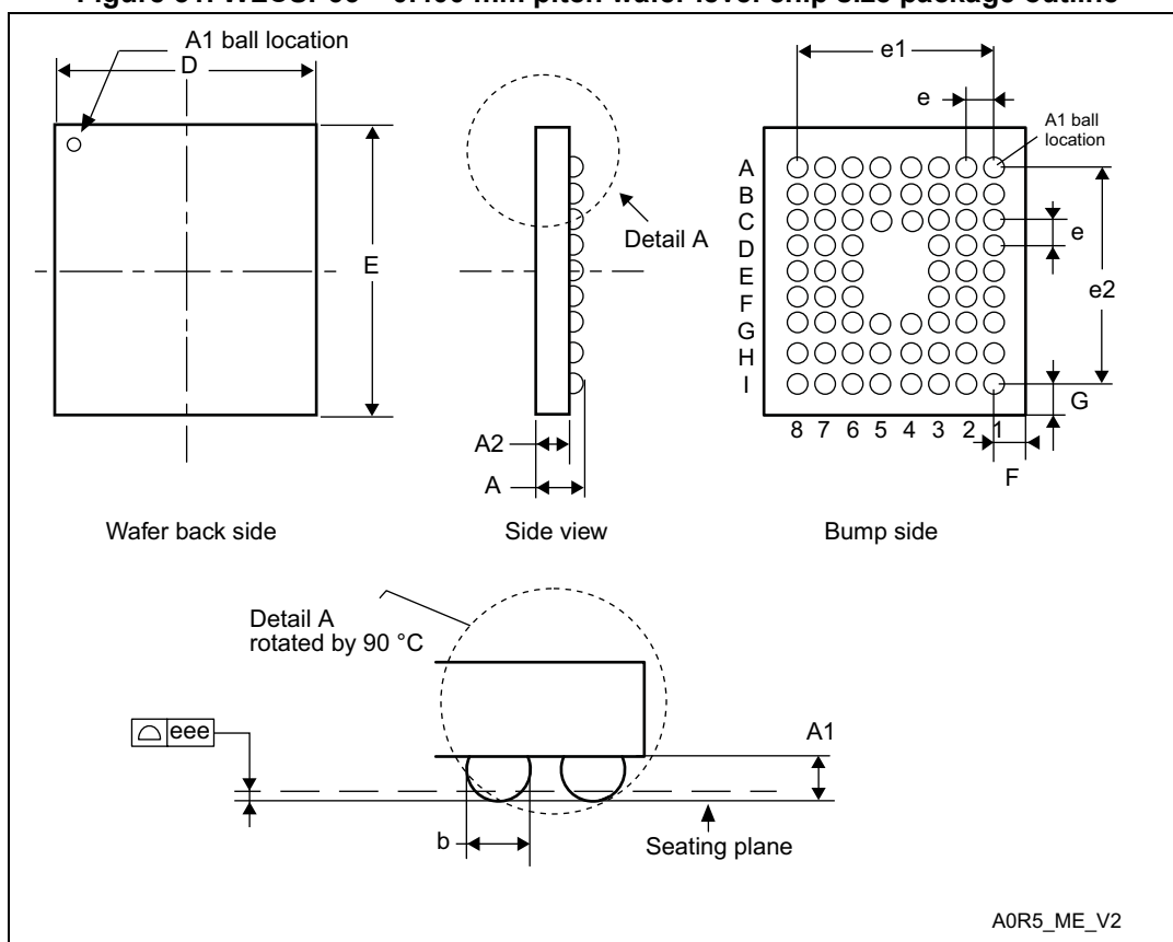
Figure 31. WLCSP66 – 0.400 mm pitch wafer level chip size package outline
