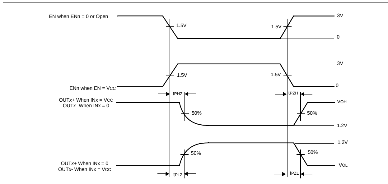
Figure 21. Driver High Impedance Delay Waveforms
