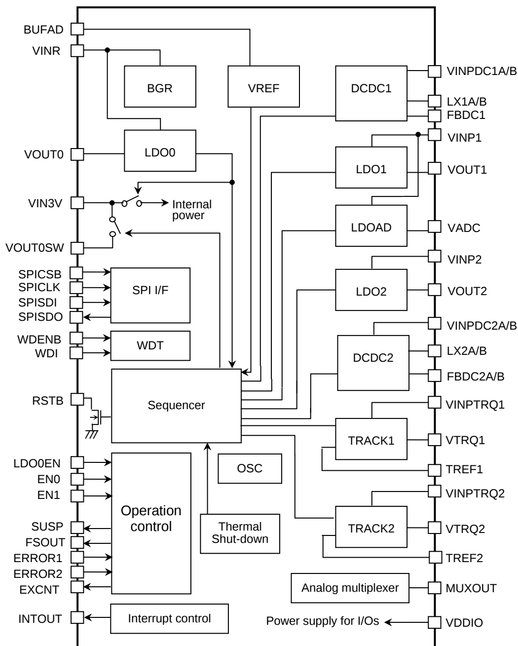
Fig. 3 The PMIC block diagram
