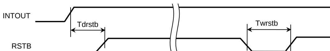
Fig. 4-9-2 RSTB timing 1
