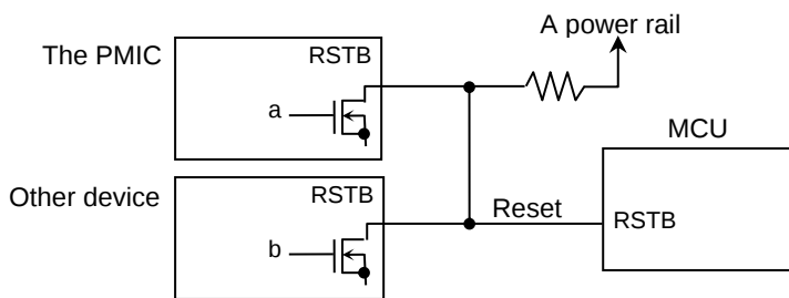
(a) Wired reset
