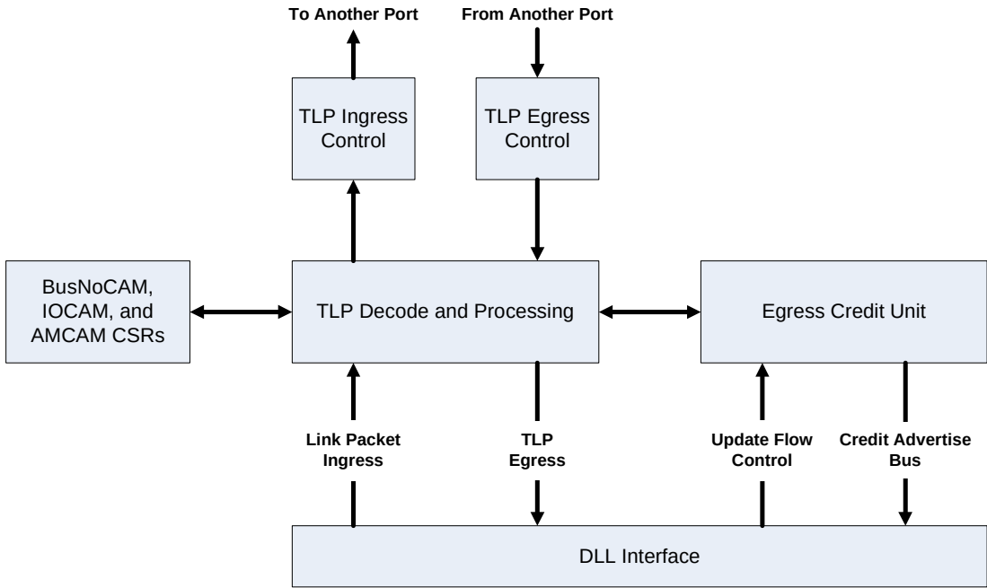
Figure 4-4. TL Controller
