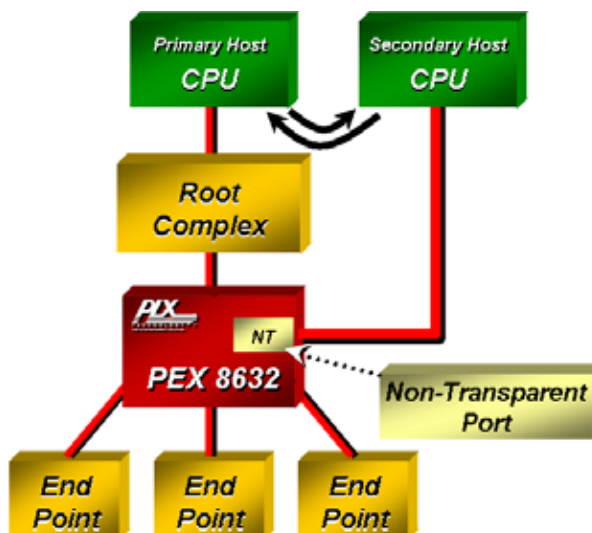
Figure 2-2. Non-Transparent Port
