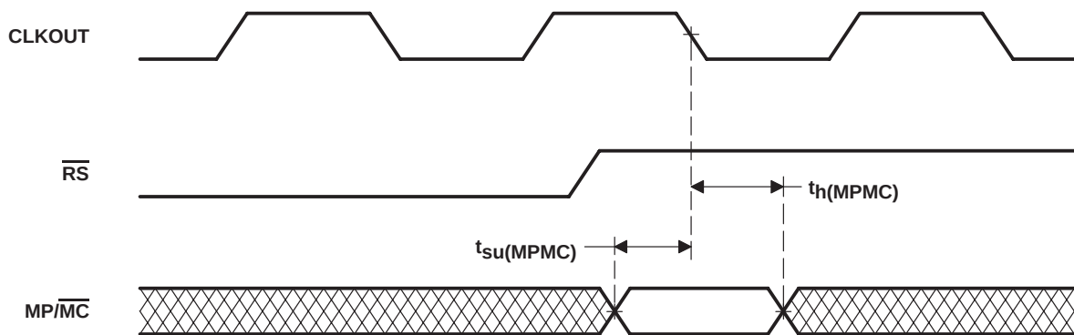
Figure 5-17. \text{MP}/\overline{\text{MC}} Timing
