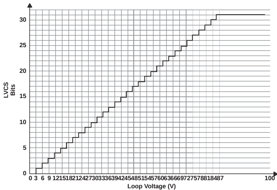
Figure 3-51. Typical Loop Voltage LVCS Transfer Function
