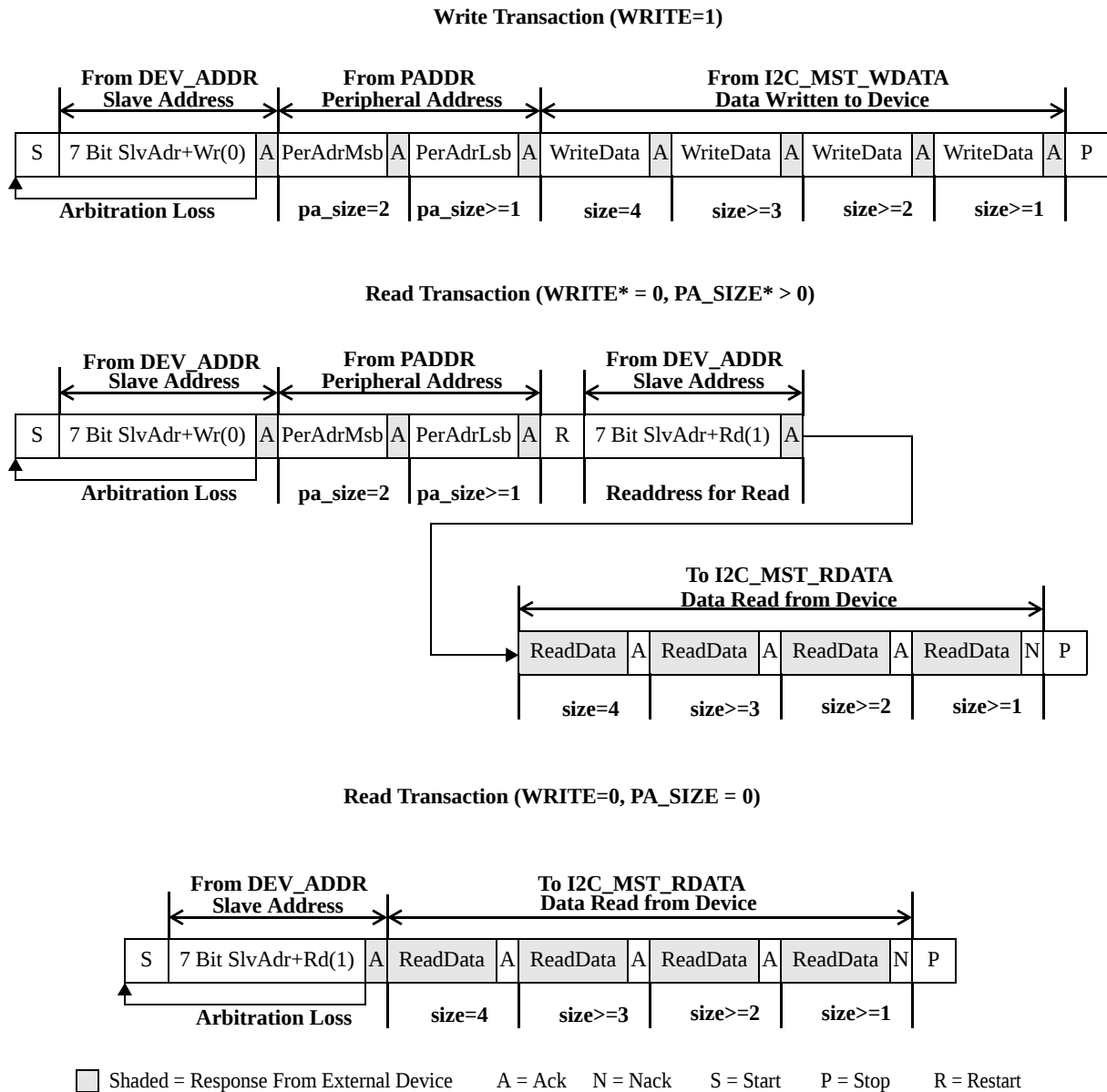
Figure 31: Software-initiated Master Transactions
