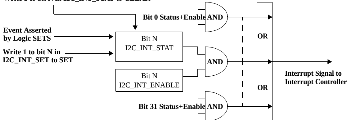
Figure 37: I 2 C Interrupt Generation
