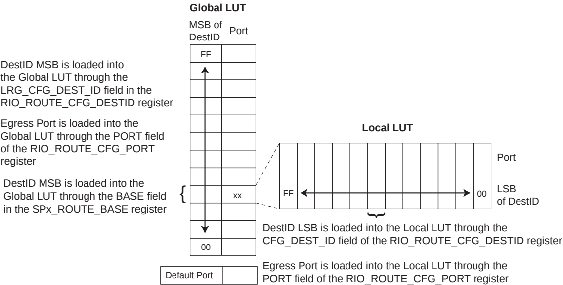
Figure 9: Hierarchical Mode
