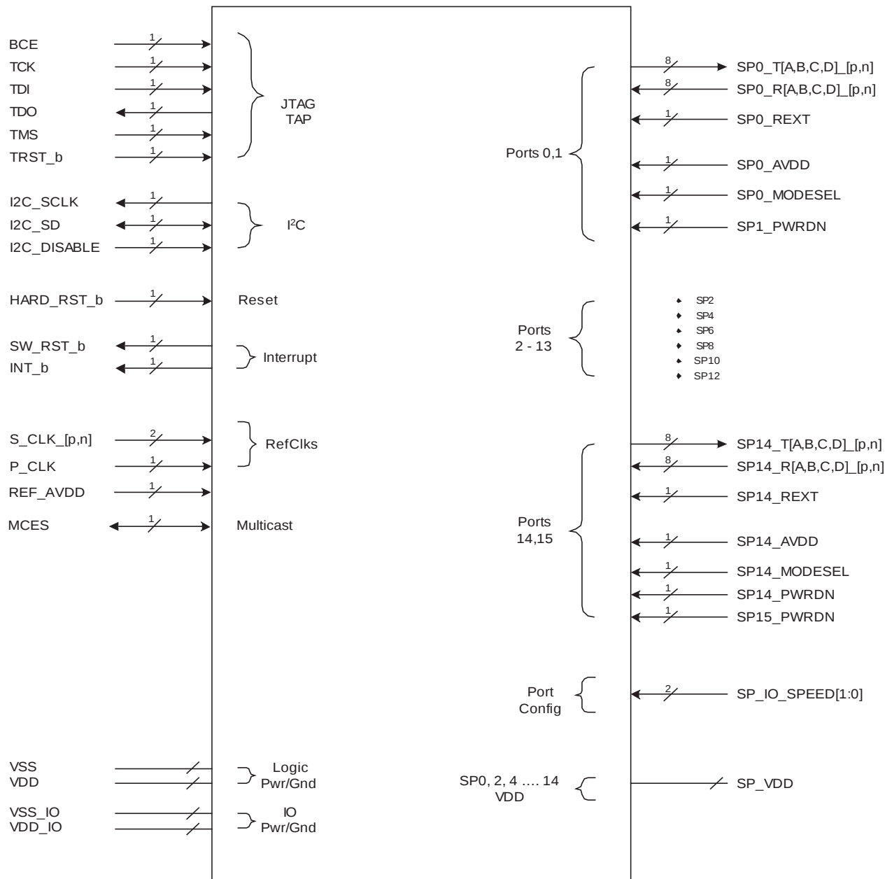
Figure 47: Signal Groupings
