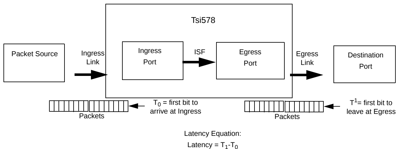
Figure 41: Latency Illustration
