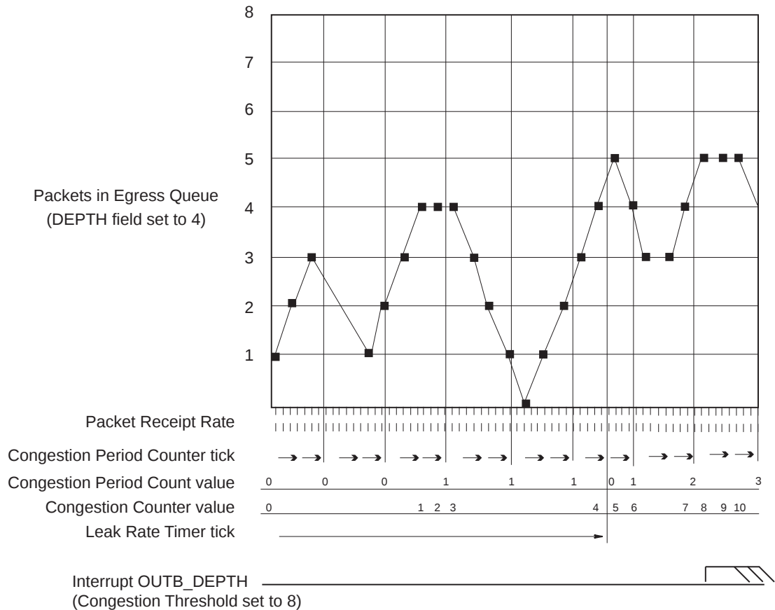
Figure 43: Congestion Example
