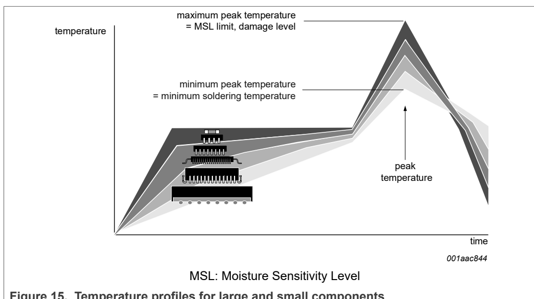
Figure 15. Temperature profiles for large and small components
