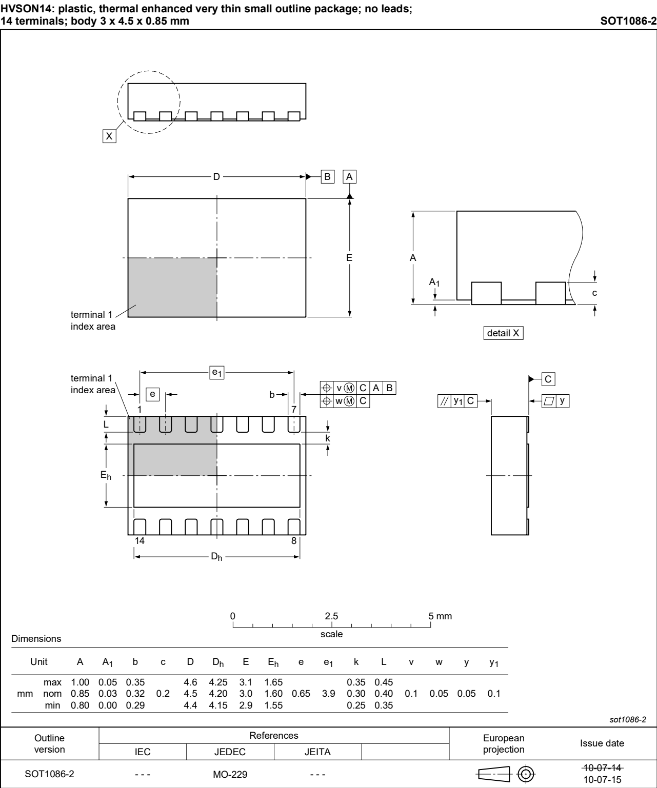
Figure 14. Package outline SOT1086-2 (HVSON14)
