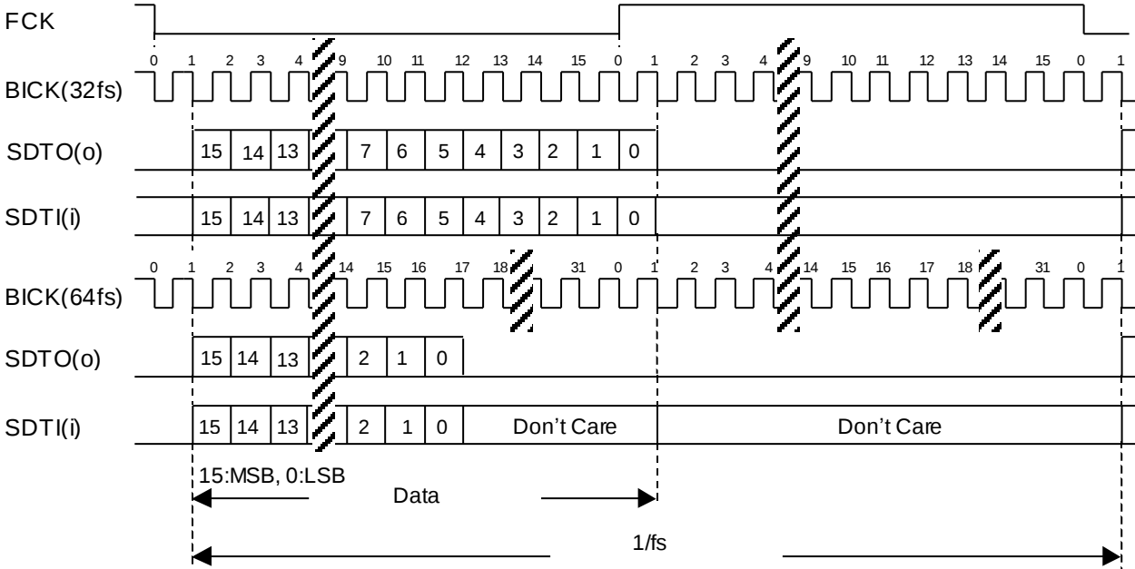
Figure 25. Mode 3 Timing
