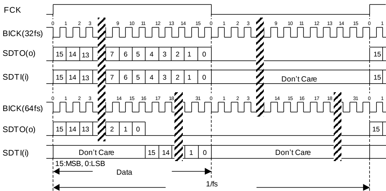
Figure 23. Mode 1 Timing
