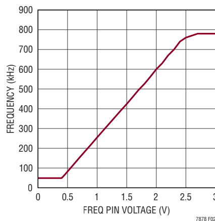
Figure 2. Relationship Between Switching Frequency and Voltage at FREQ Pin
