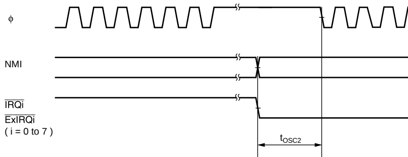
Figure 24.5 Oscillation Stabilization Timing (Exiting Software Standby Mode)
