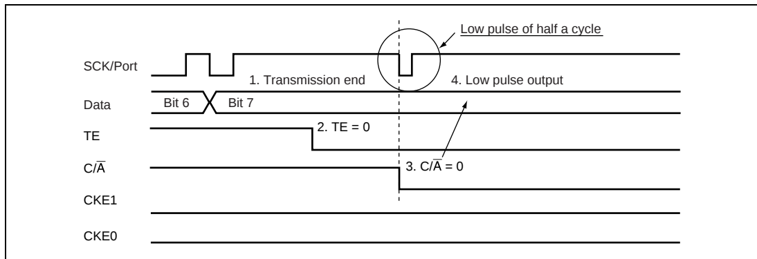
Figure 16.25 Switching from SCK Pins to Port Pins
