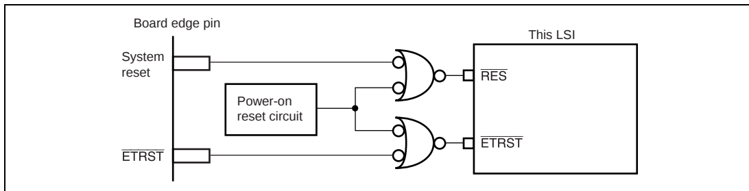
Figure 1.3 Sample Design of Reset Signals without Affection Each Other
