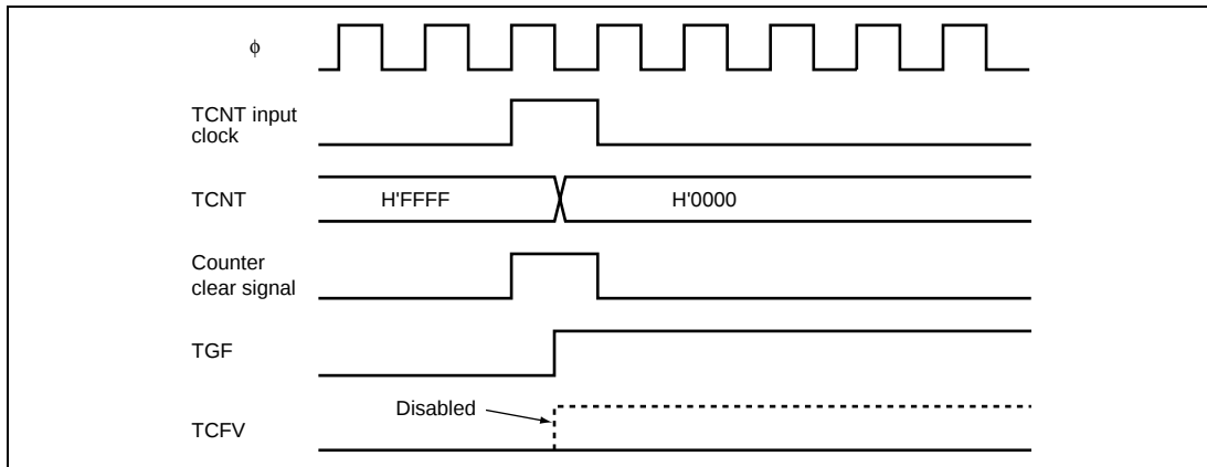
Figure 12.54 Contention between Overflow and Counter Clearing
