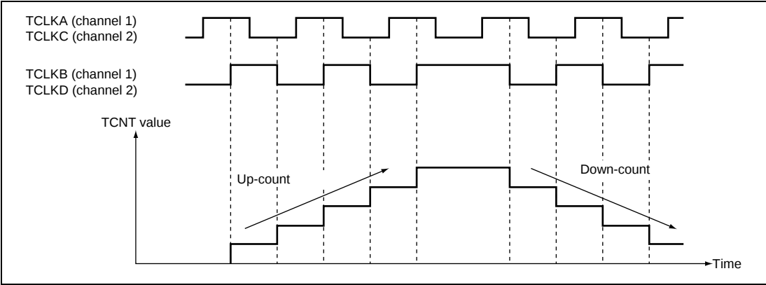
Figure 12.32 Example of Phase Counting Mode 4 Operation
