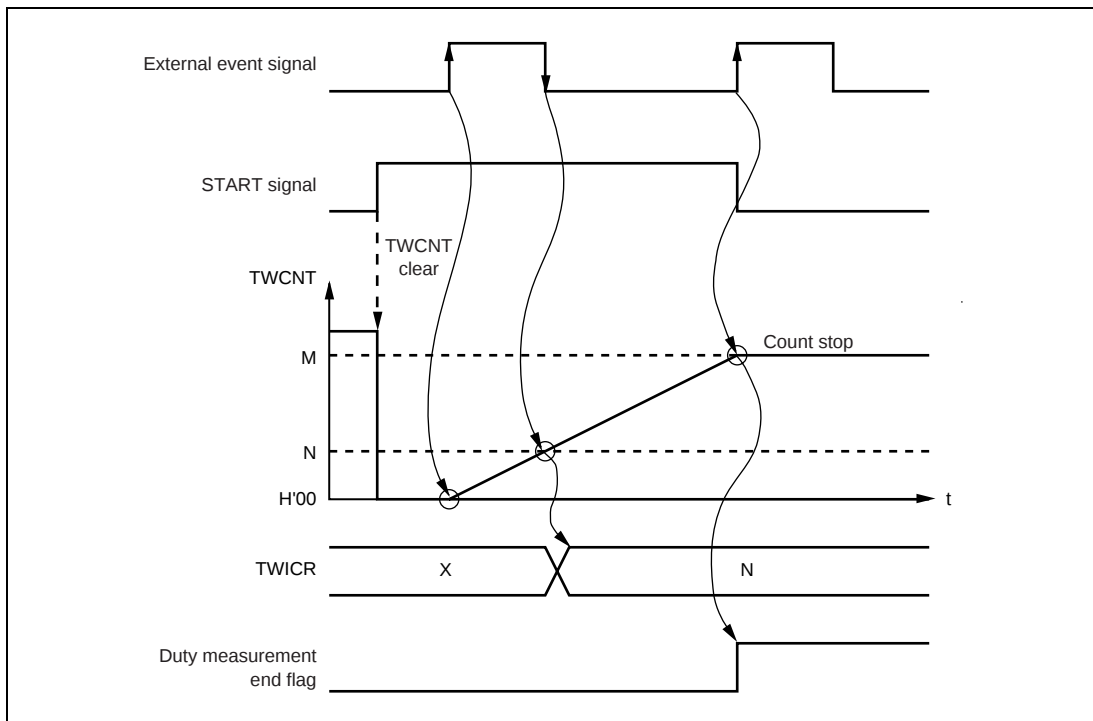
Figure 14.2 Example of Duty Measurement for External Event Signal
