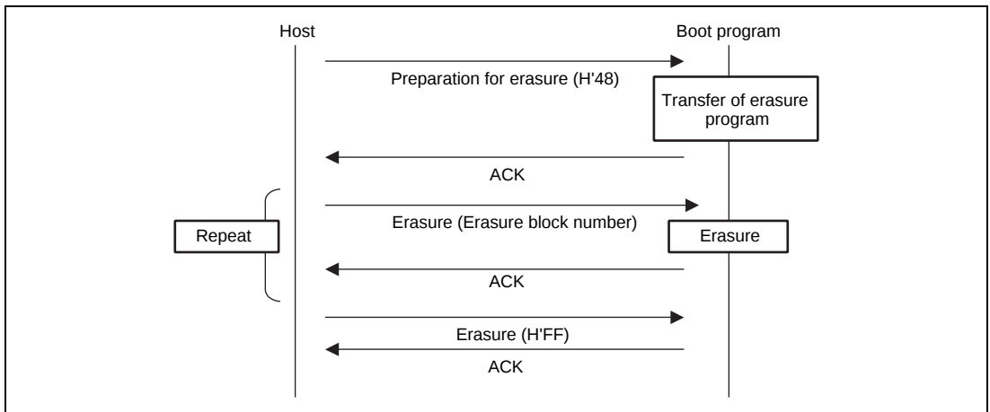
Figure 20.24 Erasure Sequence
