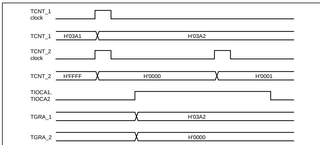
Figure 12.22 Example of Cascaded Operation (1)
