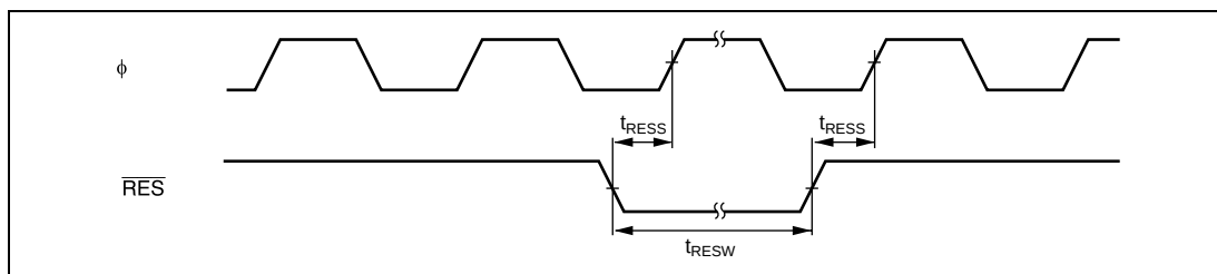
Figure 24.6 Reset Input Timing
