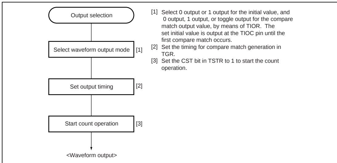
Figure 12.9 Example of Setting Procedure for Waveform Output by Compare Match
