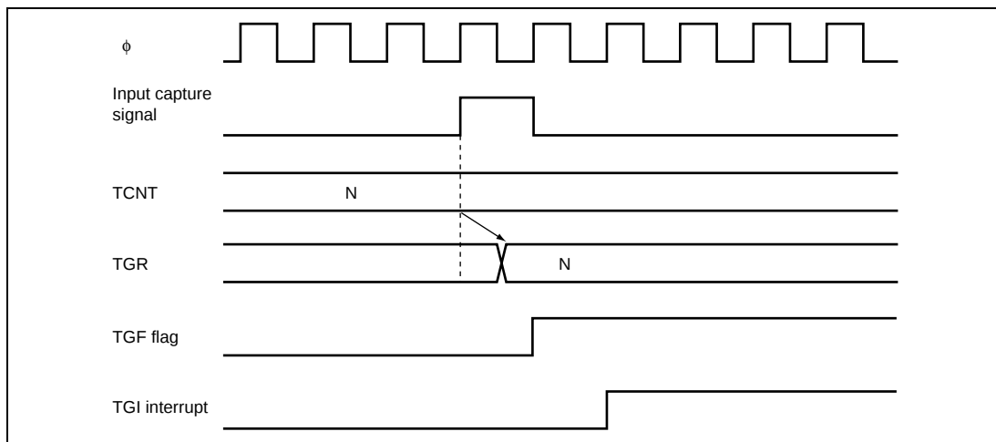
Figure 12.42 TGI Interrupt Timing (Input Capture)
