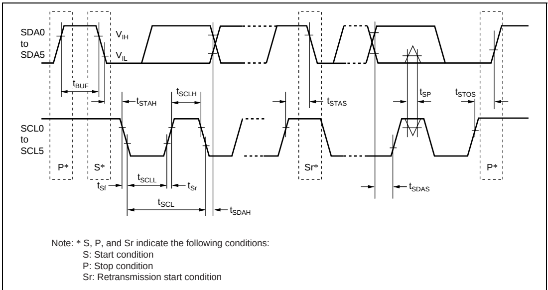
Figure 24.26 Input/Output Timing of I²C Bus Interface 3
