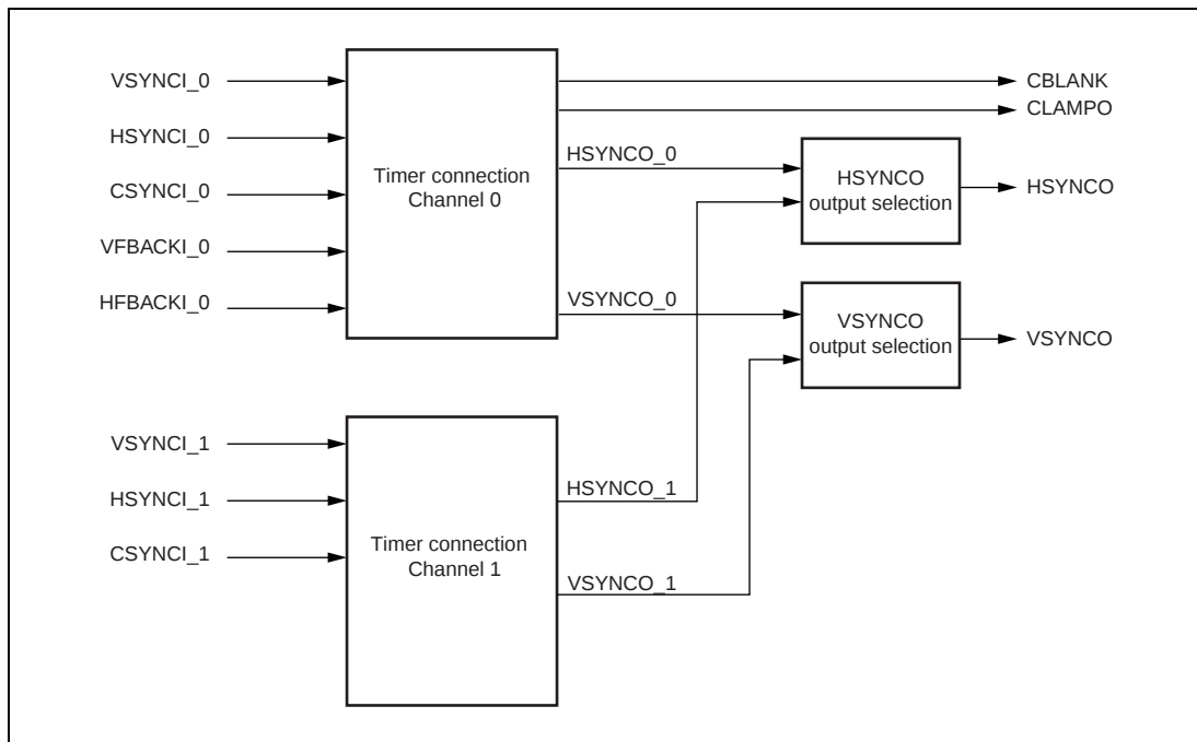
Figure 13.1 Schematic Diagram of Timer Connection
