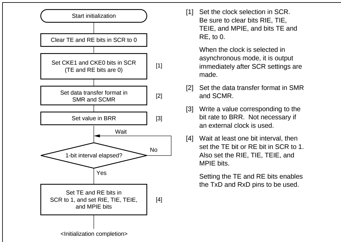
Figure 16.5 Sample SCI Initialization Flowchart
