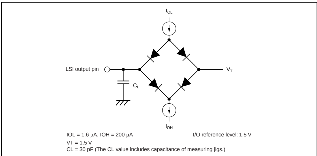
Figure 24.2 Output Load Circuit
