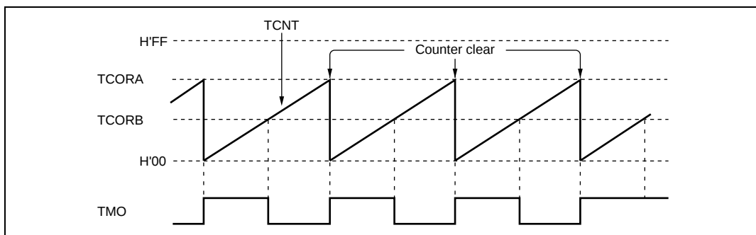
Figure 11.3 Pulse Output Example
