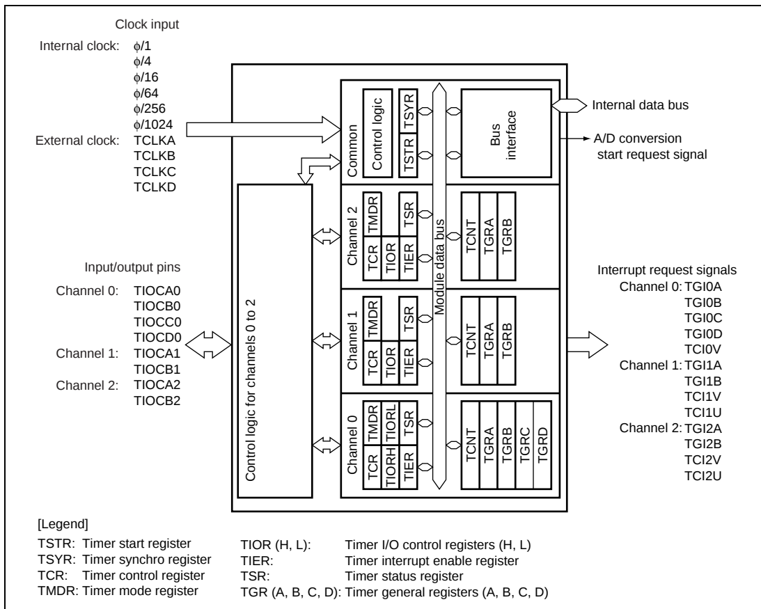
Figure 12.1 Block Diagram of TPU
