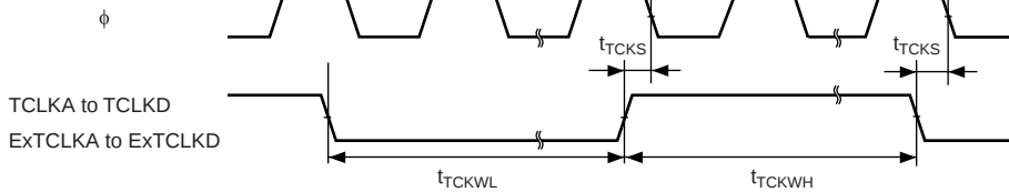
Figure 24.18 TPU Clock Input Timing
