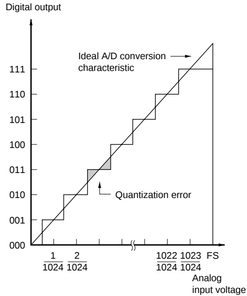
Figure 18.4 A/D Conversion Accuracy Definitions
