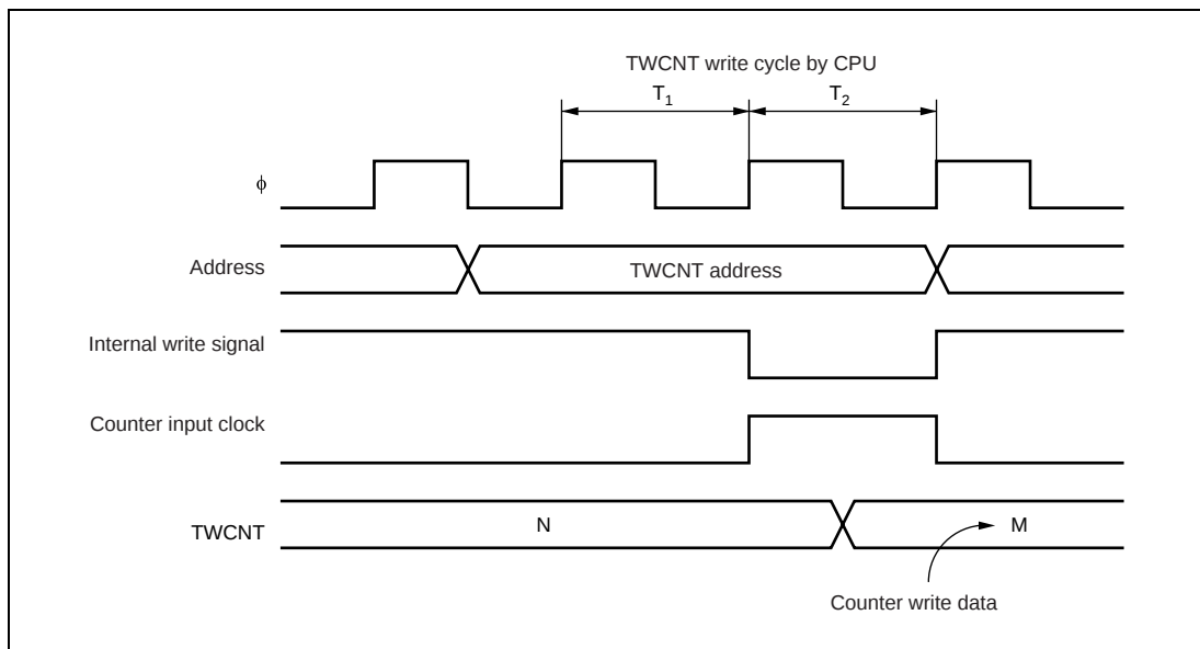
Figure 14.10 TWCNT Write-Increment Conflict
