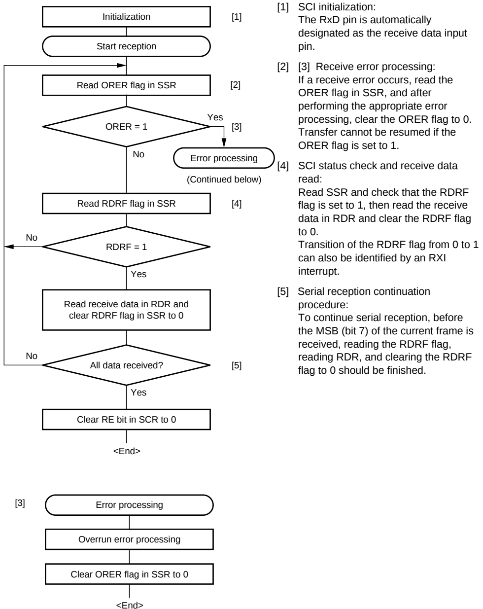
Figure 16.19 Sample Serial Reception Flowchart
