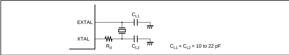
Figure 21.2 Typical Connection to Crystal Resonator
