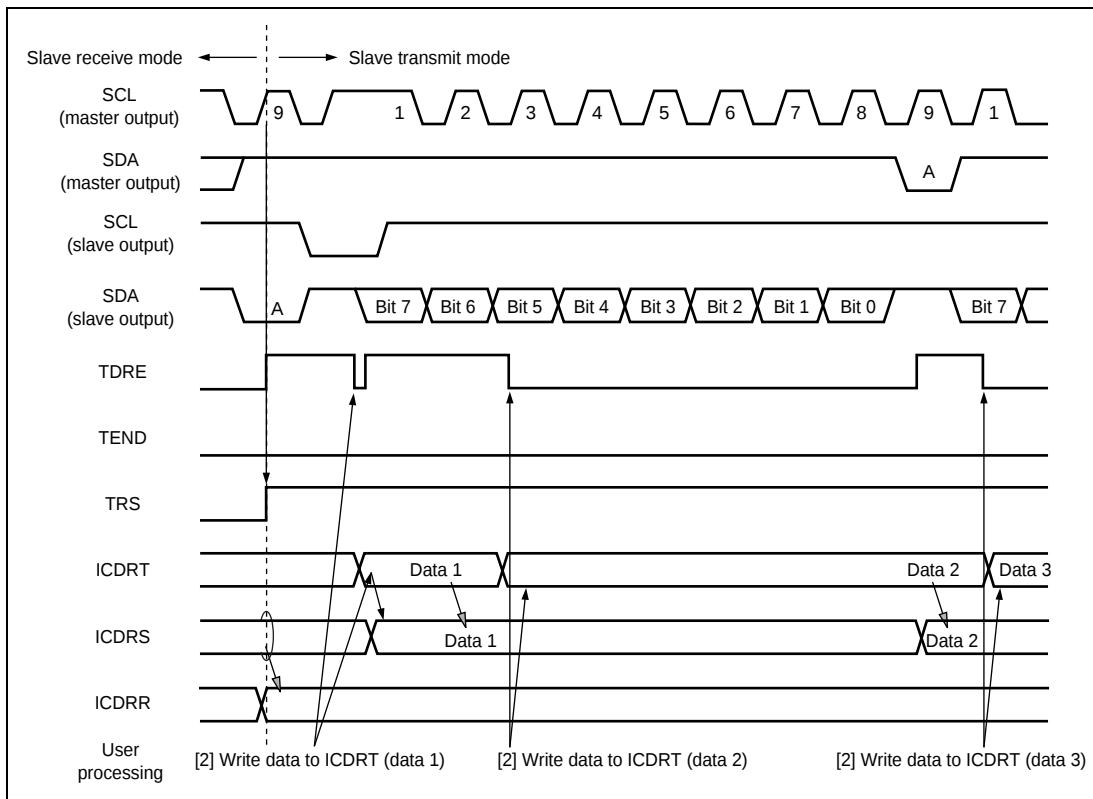
Figure 17.9 Operation Timing in Slave Transmit Mode (1)
