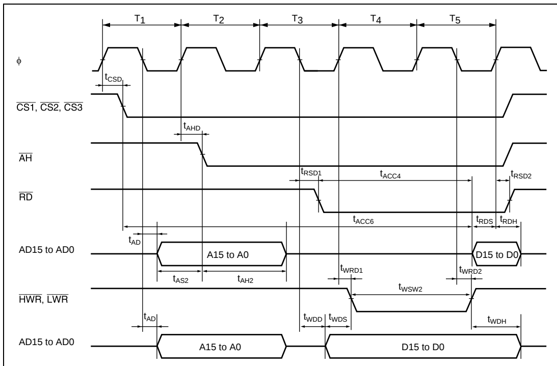
Figure 24.12 Multiplex Bus Timing/3-State Access
