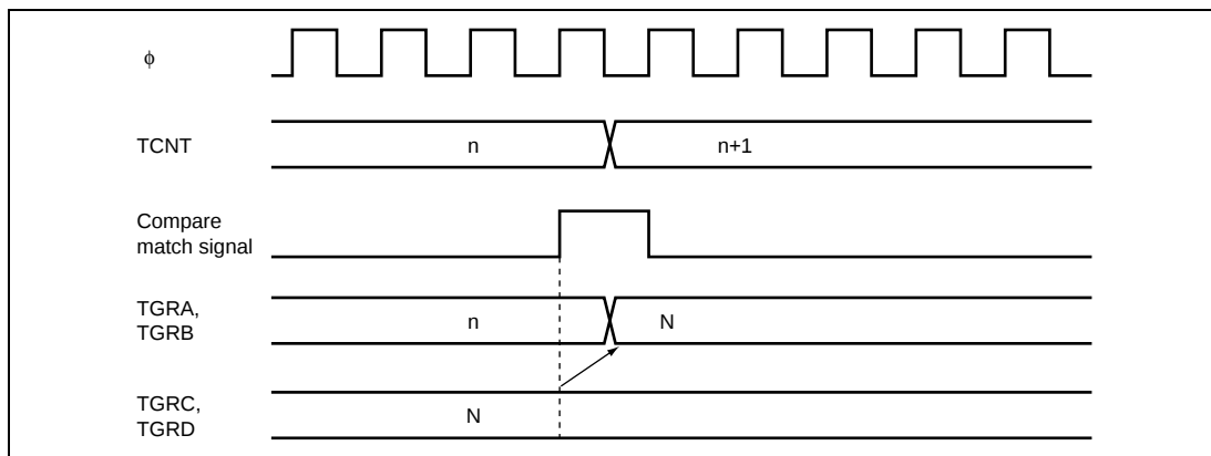
Figure 12.39 Buffer Operation Timing (Compare Match)
