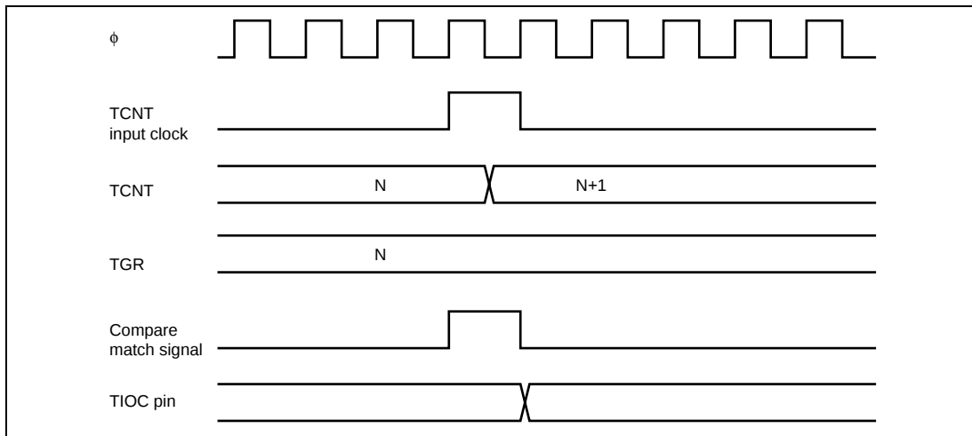
Figure 12.35 Output Compare Output Timing
