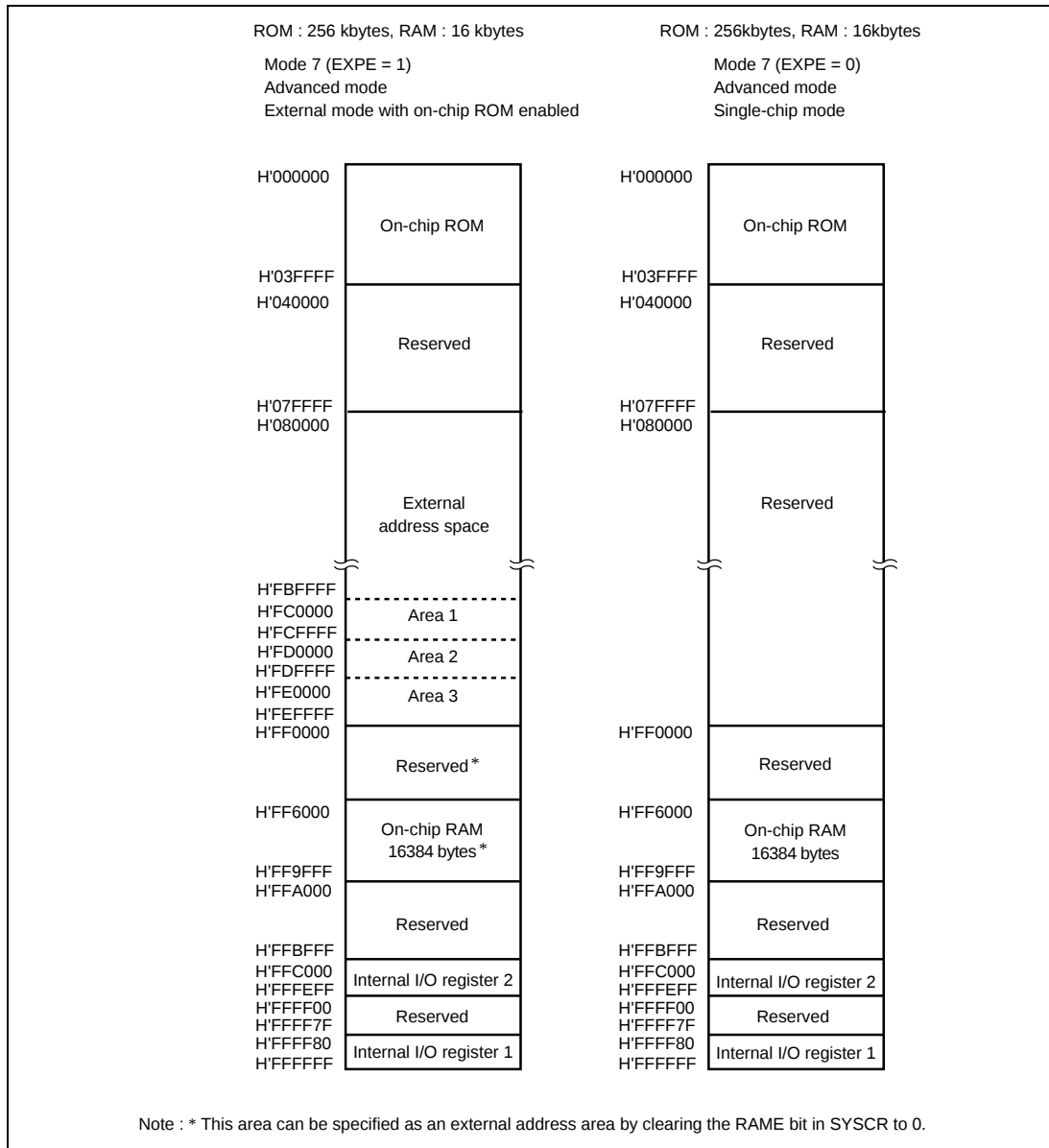
Figure 3.1 Memory Map
