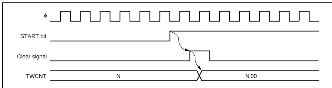
Figure 14.4 TWCNT Clear Timing by Setting START Bit
