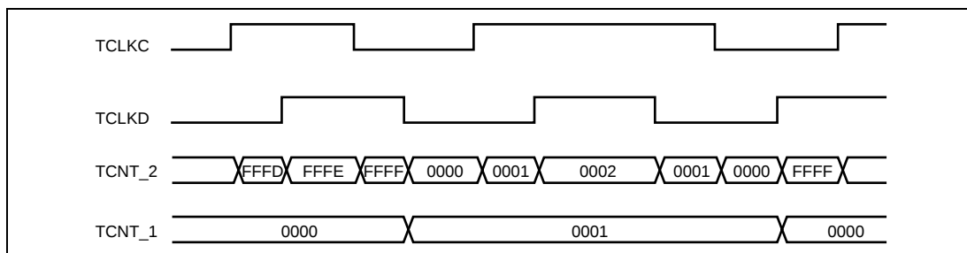
Figure 12.23 Example of Cascaded Operation (2)
