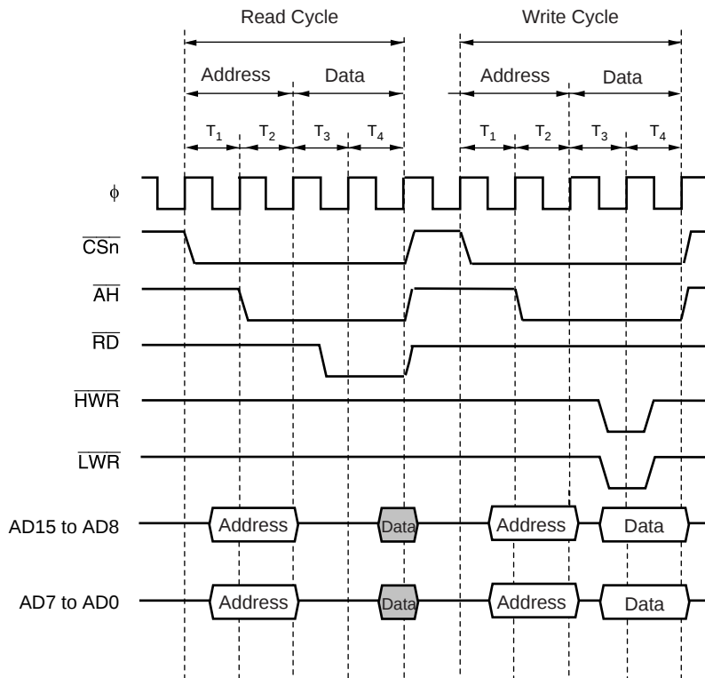
Figure 6.21 Bus Timing for 16-Bit, 2-State Data Access Space (6) (Word Access, without Address Wait)
