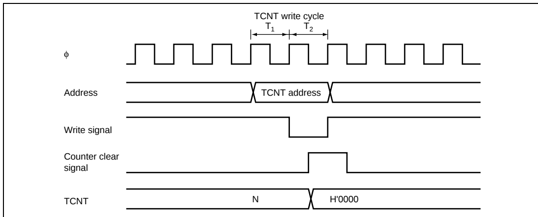
Figure 12.47 Contention between TCNT Write and Clear Operations
