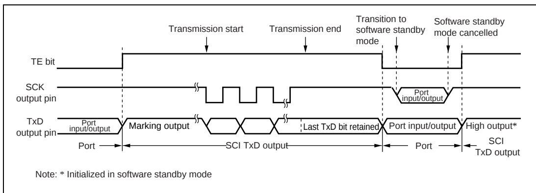
Figure 16.23 Pin States during Transmission in Clocked Synchronous Mode (Internal Clock)
