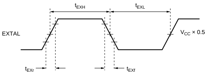
Figure 21.5 External Clock Input Timing
