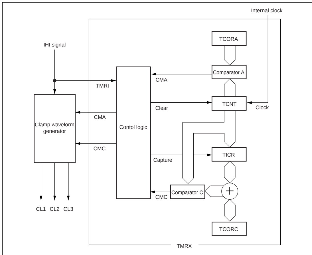
Figure 13.5 Block Diagram for Clamp Waveform Generation
