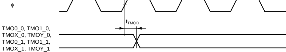
Figure 24.19 8-Bit Timer Output Timing
