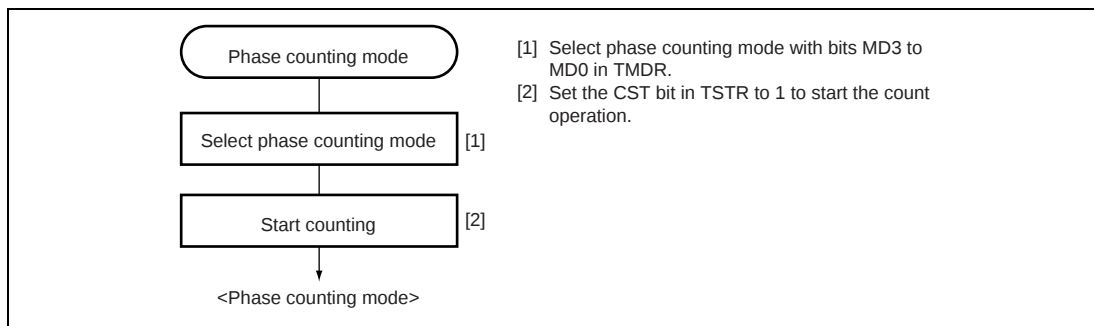
Figure 12.28 Example of Setting Procedure for Phase Counting Mode
