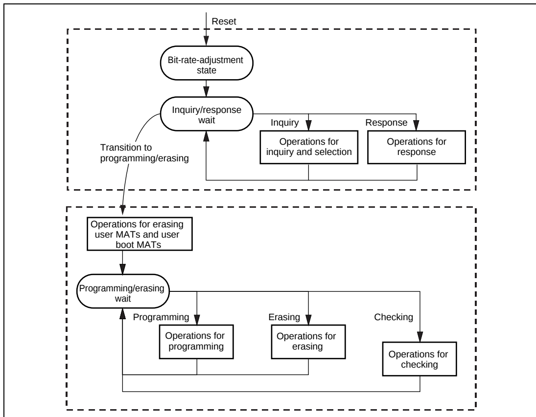
Figure 20.19 Boot Program States
