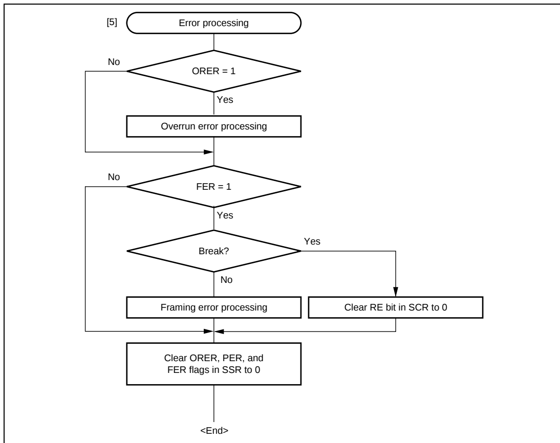
Figure 16.13 Sample Multiprocessor Serial Reception Flowchart (2)
