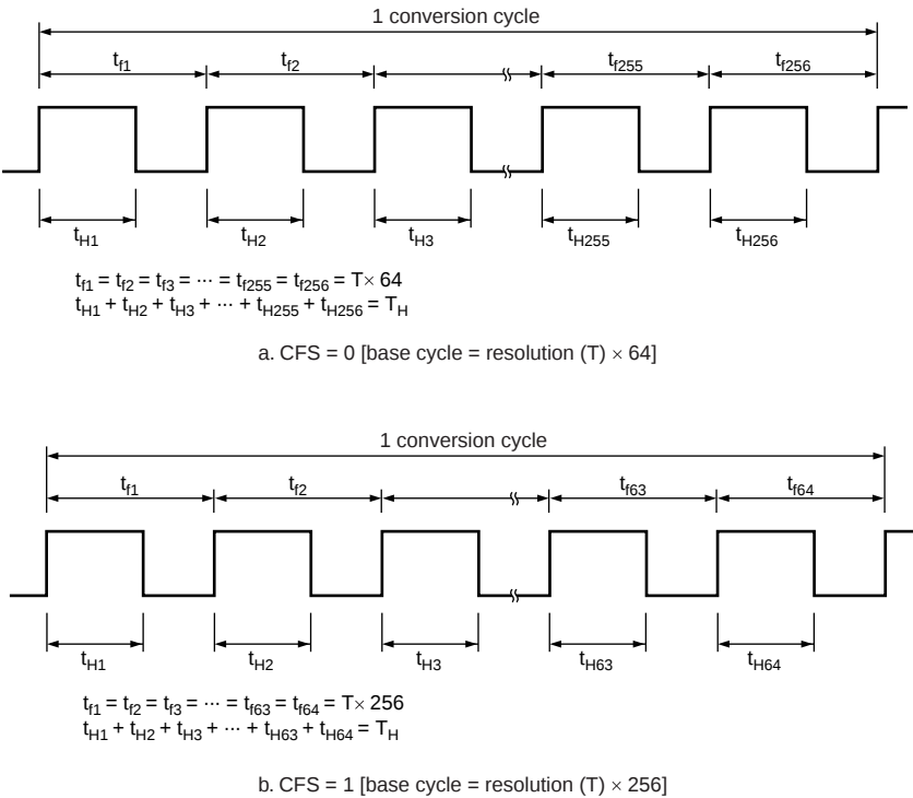
Figure 9.4 Output Waveform (OS = 1, DADR Corresponds to TH)
