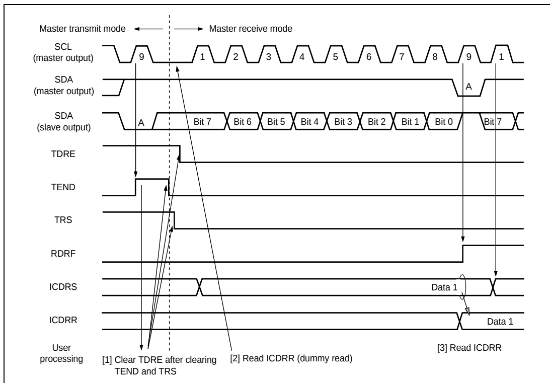
Figure 17.7 Operation Timing in Master Receive Mode (1)
