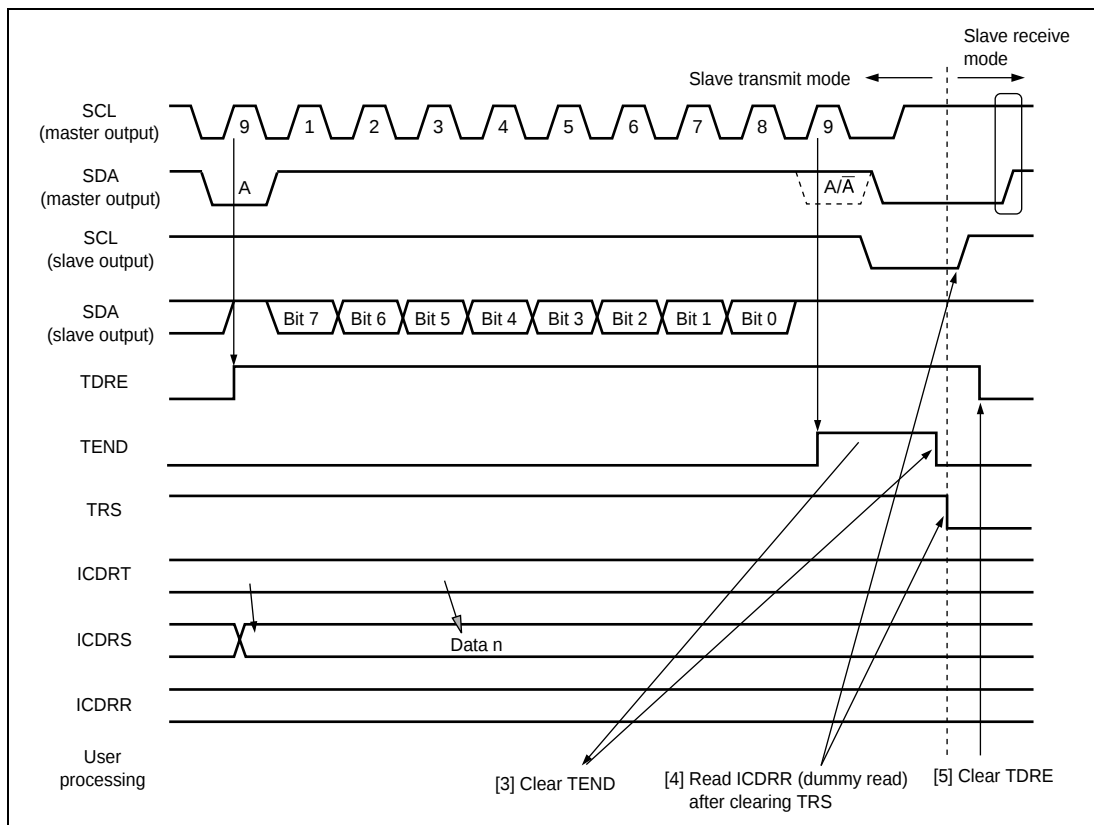
Figure 17.10 Operation Timing in Slave Transmit Mode (2)
