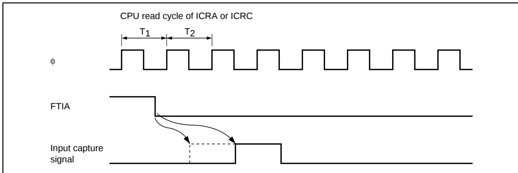
Figure 10.10 Buffered Input Capture Timing (BUFEA = 1)
