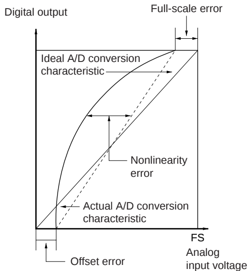
Figure 18.5 A/D Conversion Accuracy Definitions
