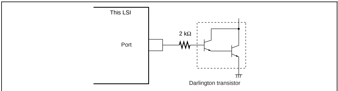
Figure 24.1 Darlington Transistor Drive Circuit (Example)
