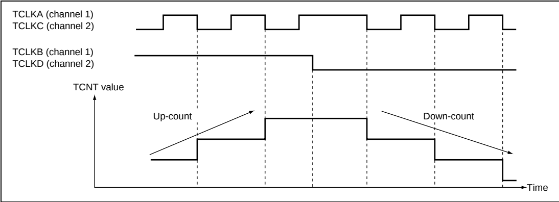
Figure 12.30 Example of Phase Counting Mode 2 Operation
