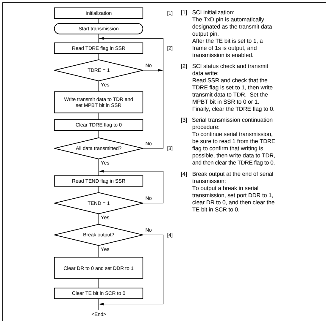
Figure 16.11 Sample Multiprocessor Serial Transmission Flowchart
