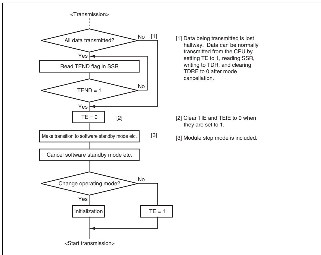
Figure 16.21 Sample Flowchart for Mode Transition during Transmission
