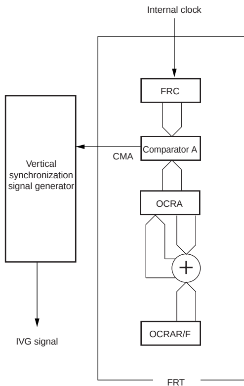
Figure 13.14 Block Diagram for IVG Signal Generation
