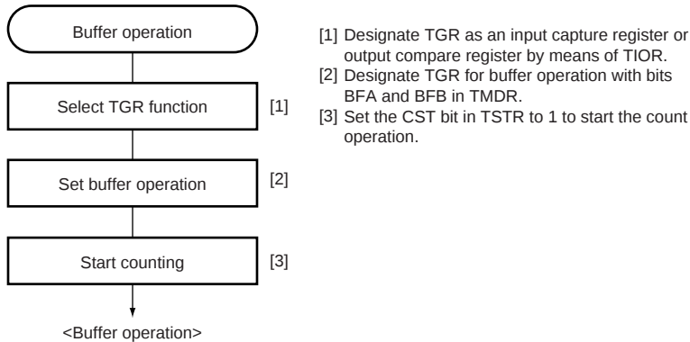
Figure 12.18 Example of Buffer Operation Setting Procedure
