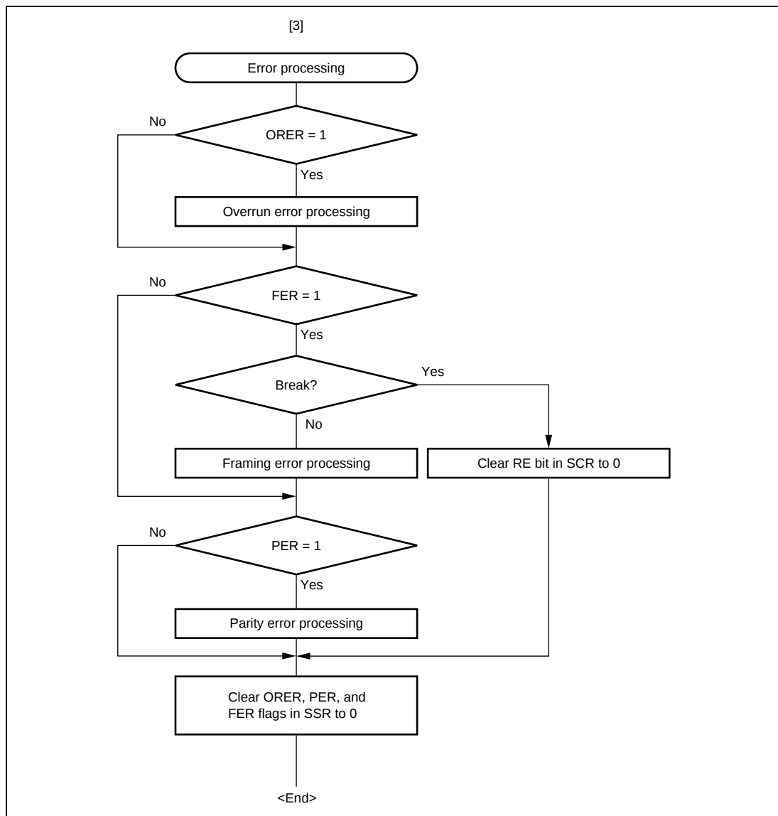
Figure 16.9 Sample Serial Reception Flowchart (2)
