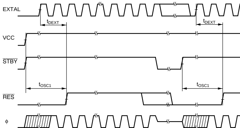
Figure 24.4 Oscillation Stabilization Timing
