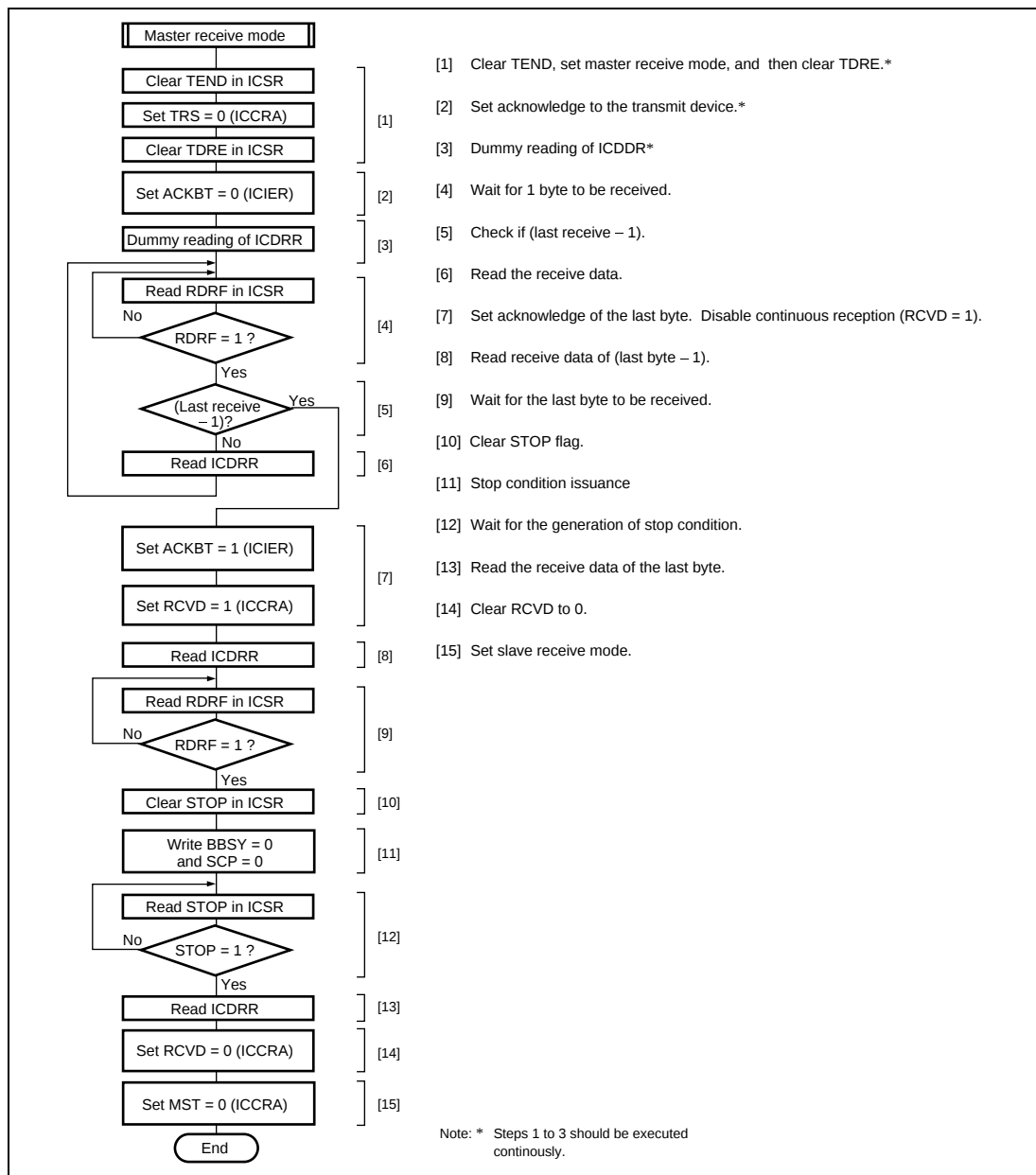
Figure 17.15 Sample Flowchart for Master Receive Mode
