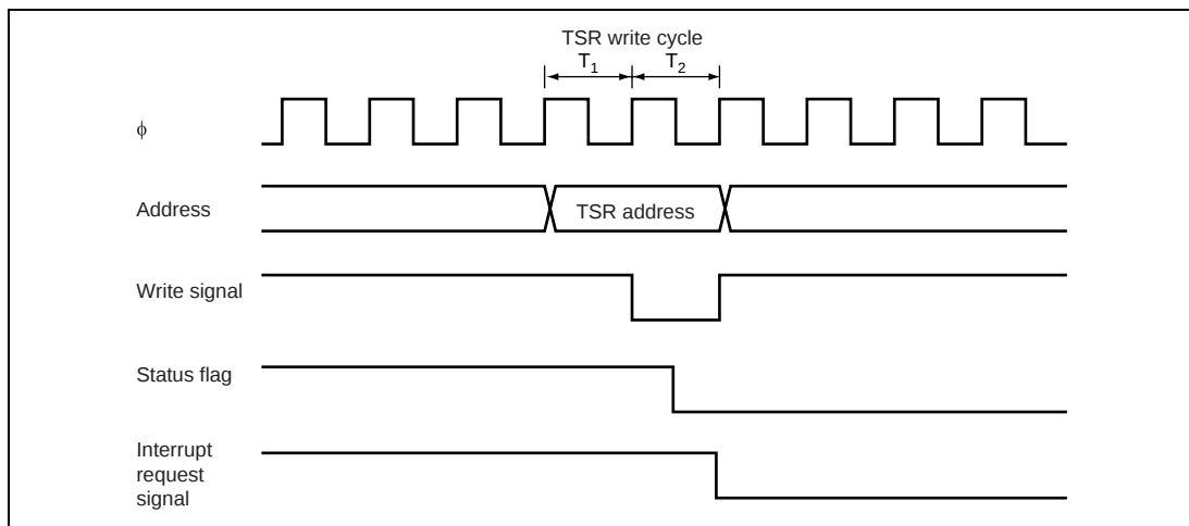
Figure 12.45 Timing for Status Flag Clearing by CPU
