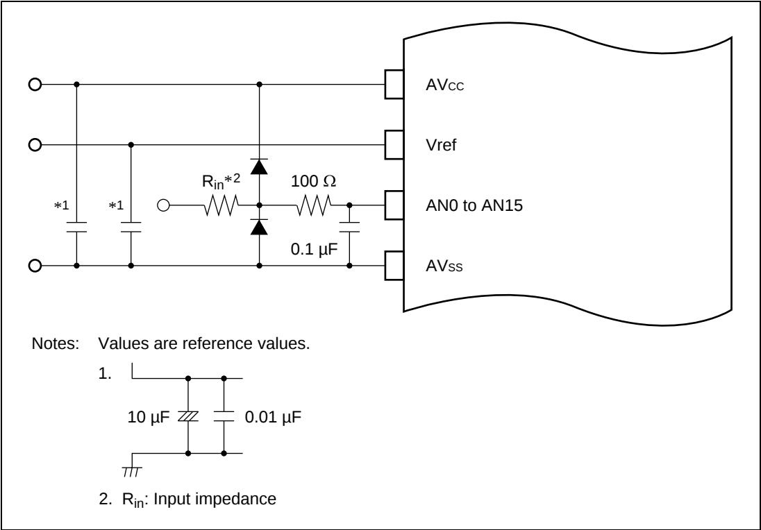
Figure 18.7 Example of Analog Input Protection Circuit
