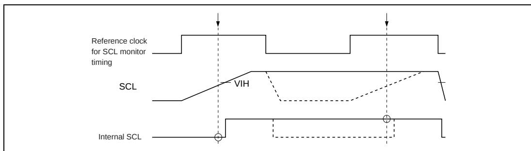
Figure 17.18 Timing of Bit Synchronous Circuit
