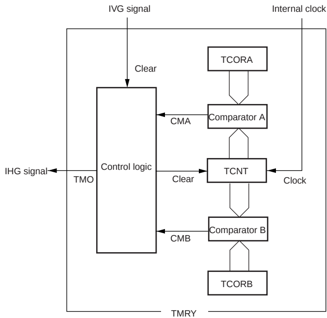
Figure 13.15 Block Diagram for IHG Signal Generation
