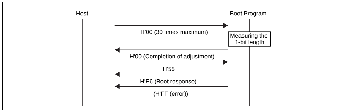
Figure 20.20 Bit-Rate-Adjustment Sequence
