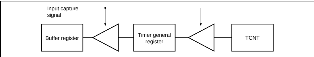
Figure 12.17 Input Capture Buffer Operation
