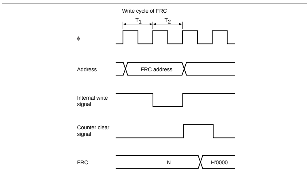
Figure 10.17 FRC Write-Clear Conflict
