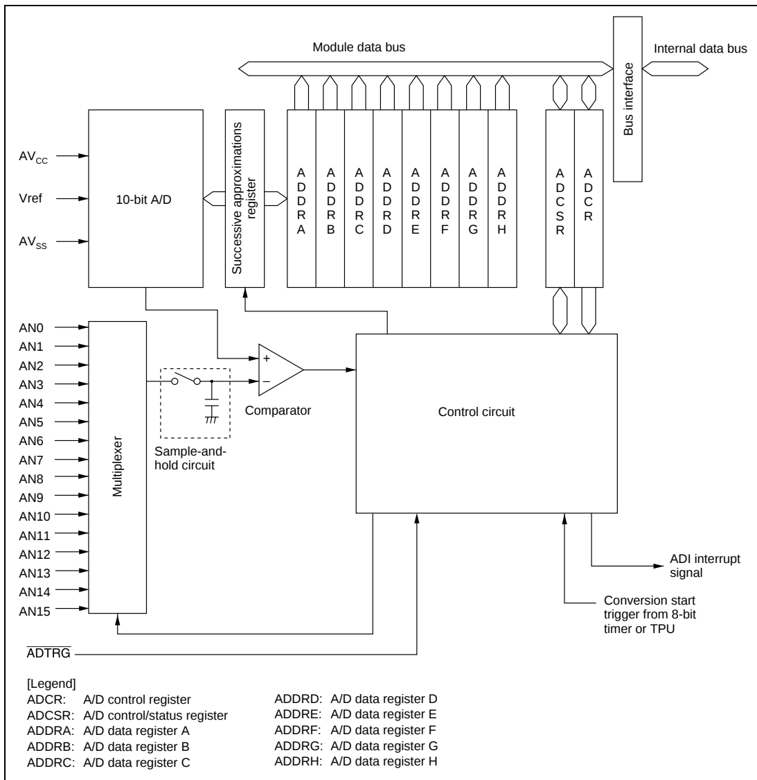
Figure 18.1 Block Diagram of A/D Converter
