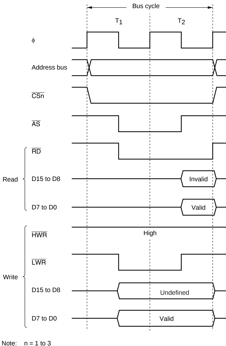
Figure 6.8 Bus Timing for 16-Bit, 2-State Access Space (Odd Byte Access)
