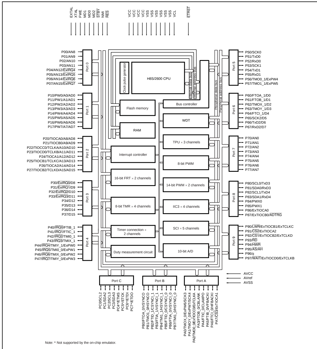
Figure 1.1 Internal Block Diagram of H8S/2437 Group
