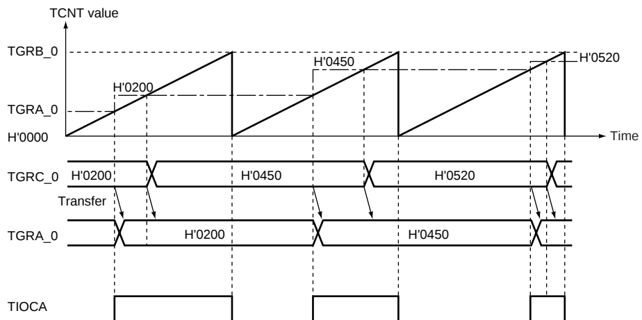
Figure 12.19 Example of Buffer Operation (1)
