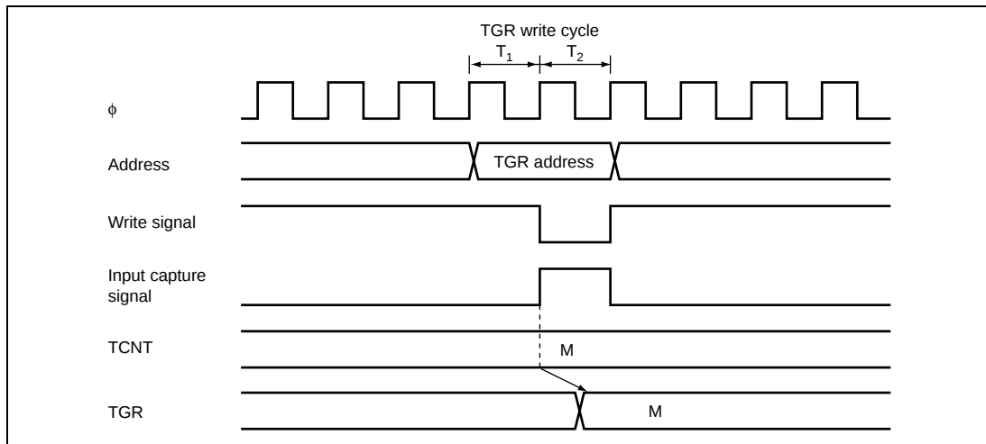
Figure 12.52 Contention between TGR Write and Input Capture
