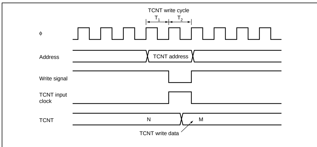
Figure 12.48 Contention between TCNT Write and Increment Operations
