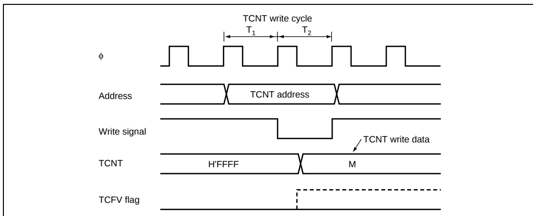
Figure 12.55 Contention between TCNT Write and Overflow
