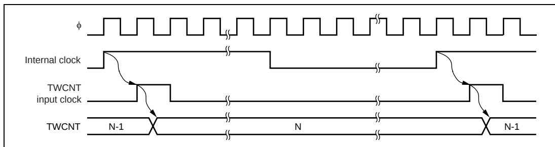
Figure 14.3 TWCNT Count Timing
