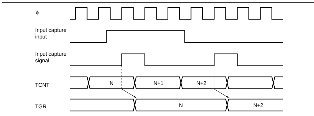
Figure 12.36 Input Capture Input Signal Timing
