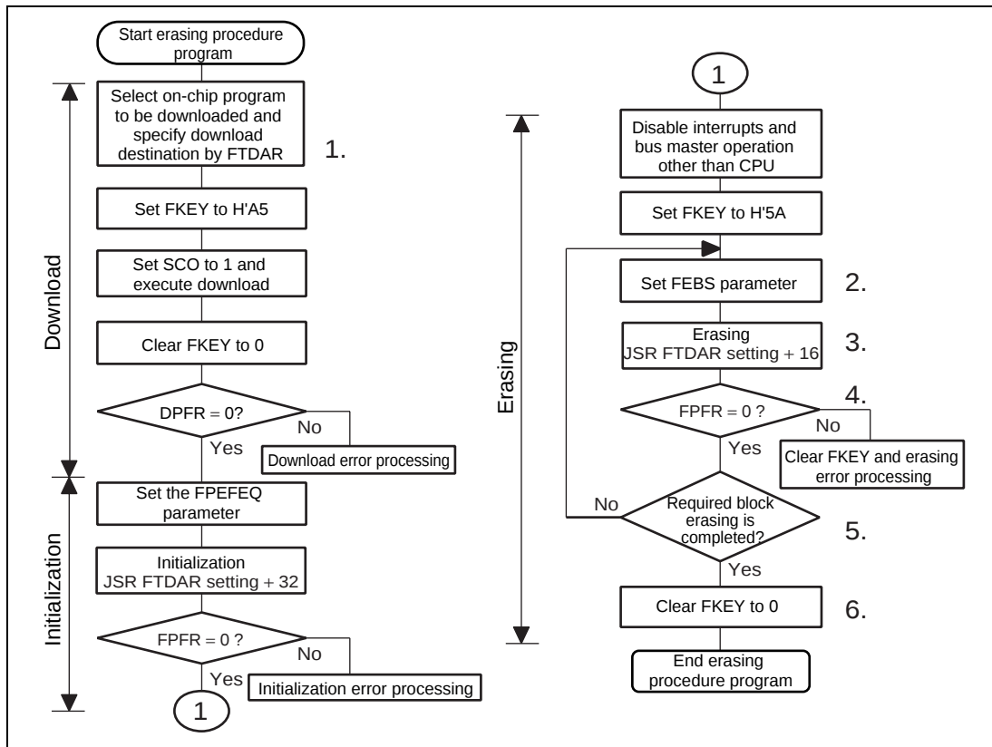
Figure 20.12 Erasing Procedure
