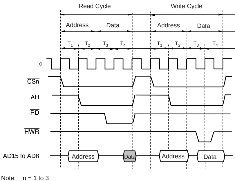
Figure 6.14 Bus Timing for 8-Bit, 2-State Data Access Space (Without Address Wait)
