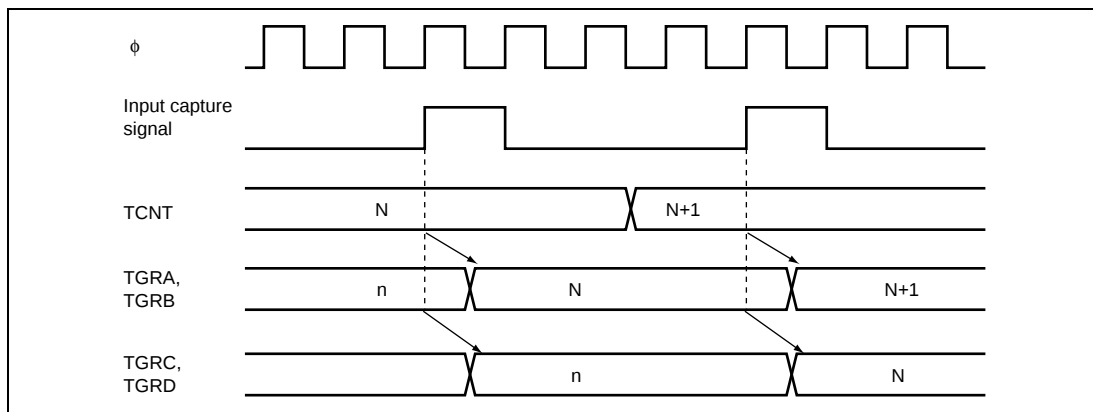
Figure 12.40 Buffer Operation Timing (Input Capture)
