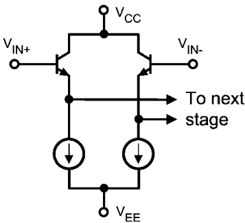
FIGURE 1. Input Stage
