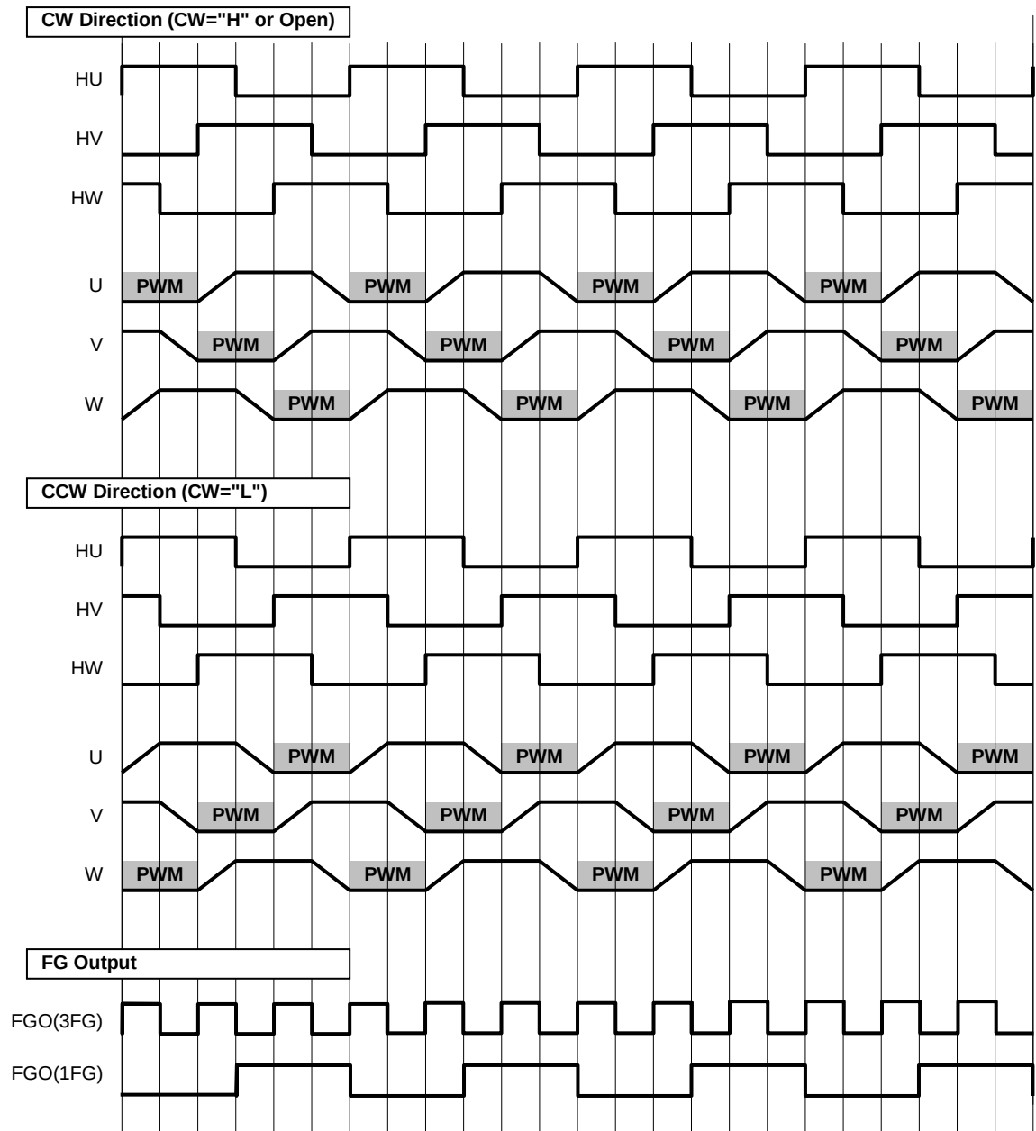
Figure 4. Timing Chart
