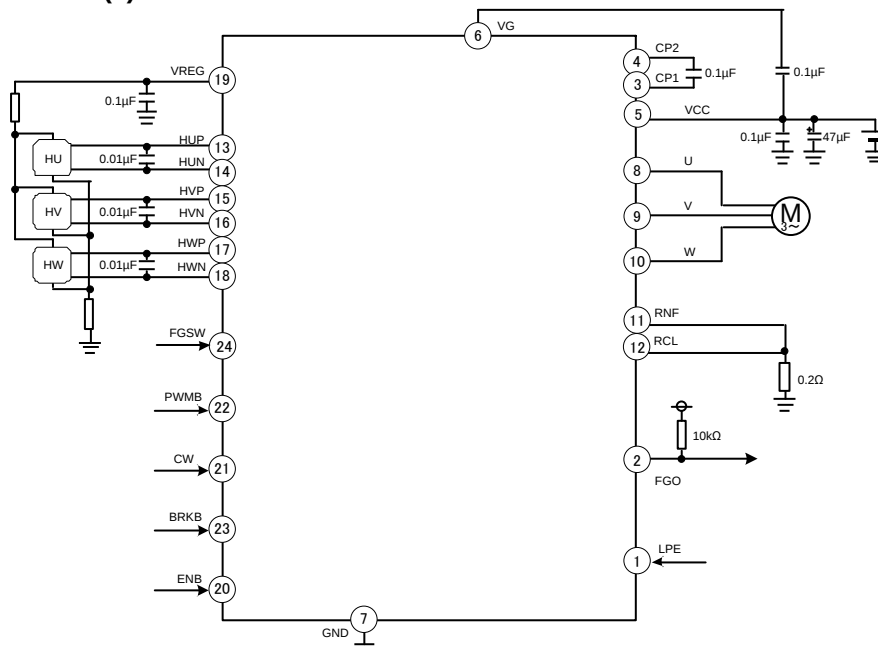
Figure 1. Application Circuit
