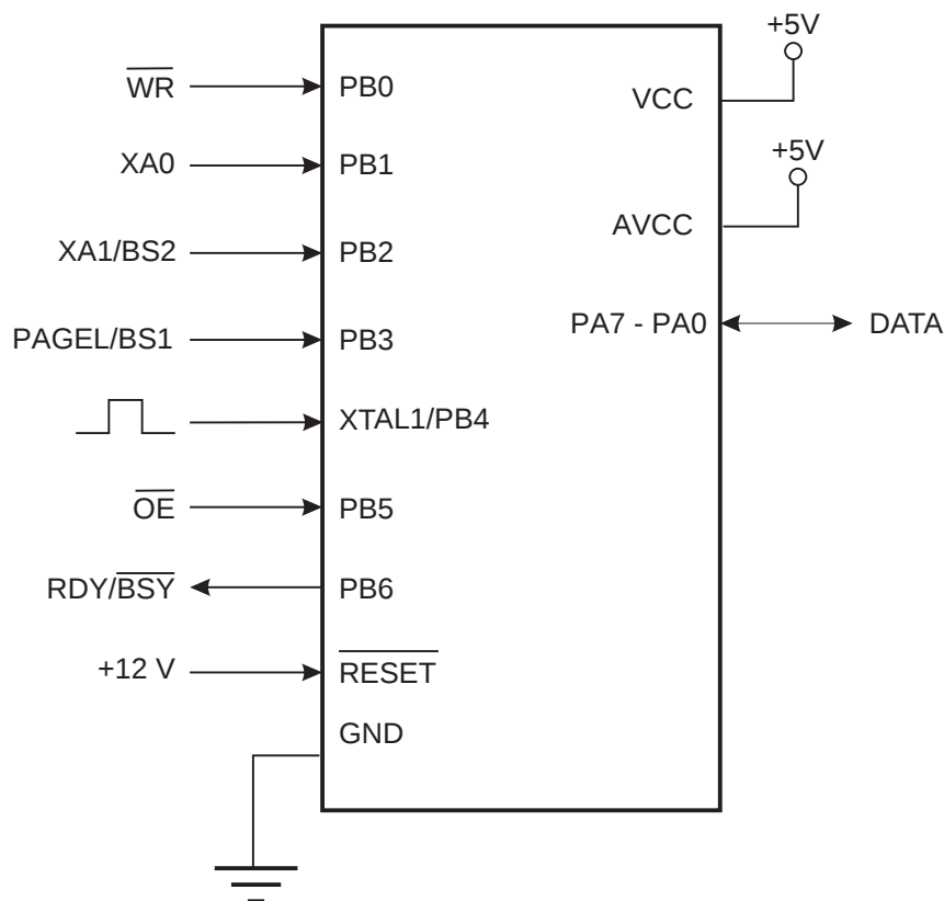
Figure 18-3. Parallel Programming.
