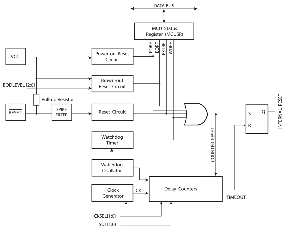
Figure 8-1. Reset Logic
