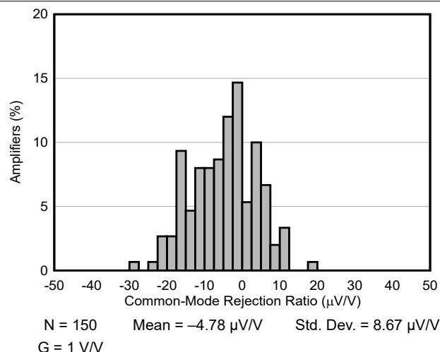
Figure 7-9. Typical CMRR Distribution at G = 1 V/V
