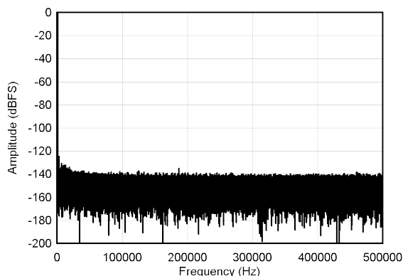
Figure 9-8. Noise Performance FFT Plots for G = 1\text{ V/V}
