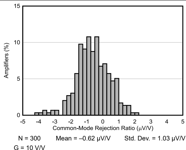
Figure 7-10. Typical CMRR Distribution at G = 10 V/V
