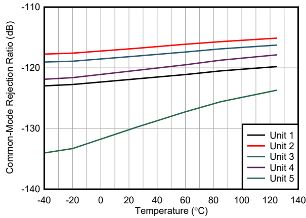
Figure 7-19. CMRR vs Temperature
