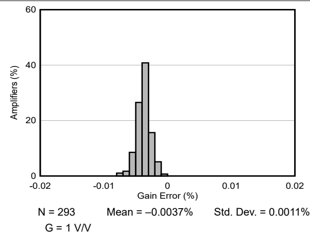
Figure 7-12. Typical Gain Error Distribution at G = 1 V/V
