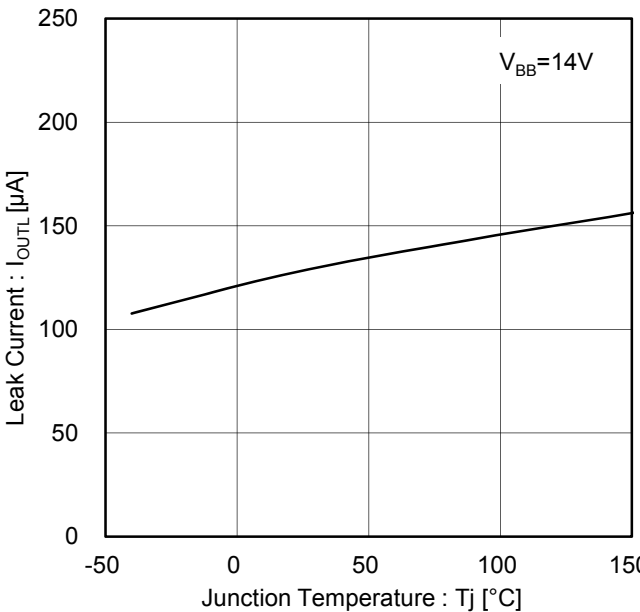
Figure 15. Leak Current vs. Temperature
