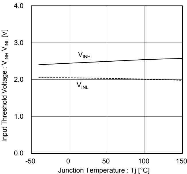
Figure 11. Input Threshold Voltage vs. Temperature
