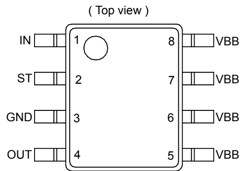
Figure 2. Pin Configurations
