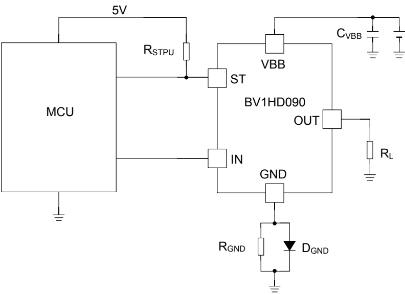
Figure 40. Application Circuits
