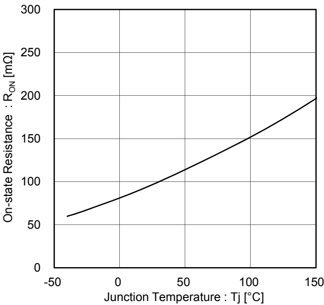
Figure 14. On-state Resistance vs. Temperature
