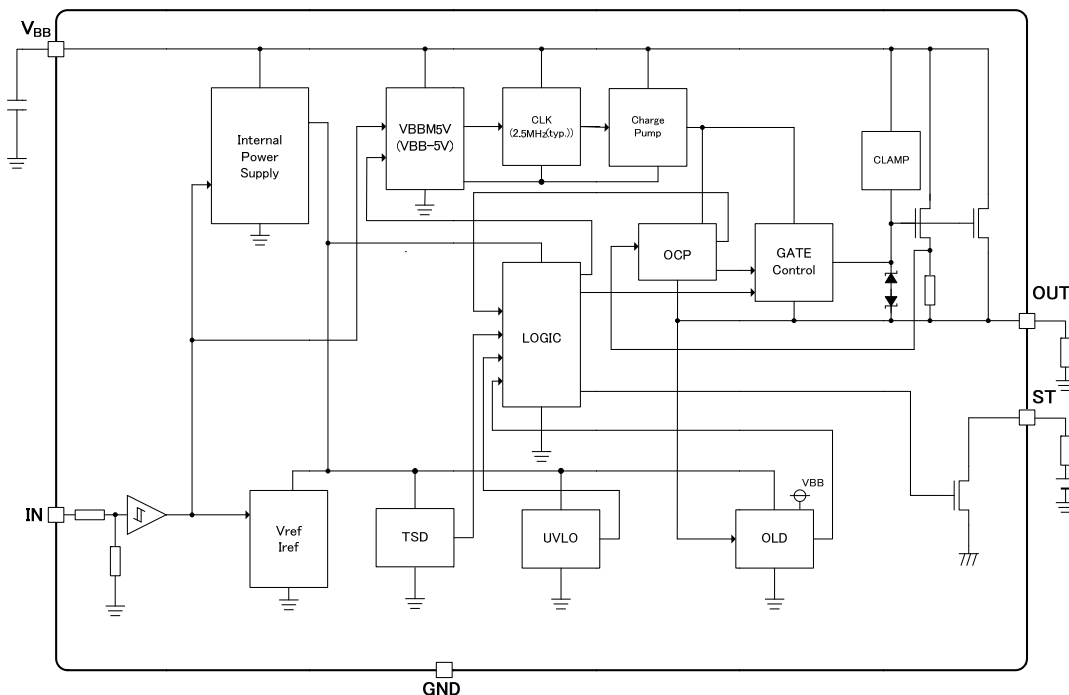
Figure 1. Block Diagram
