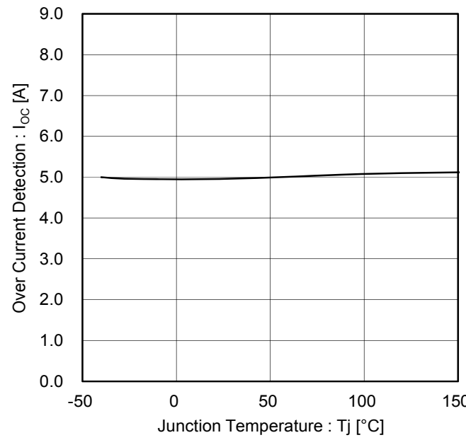
Figure 23. Overcurrent Detection vs. Temperature
