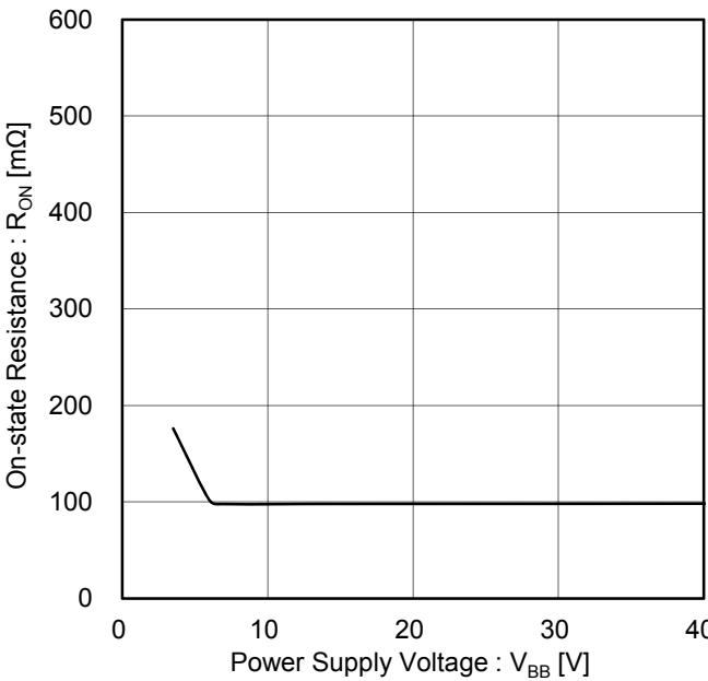
Figure 13. On-state Resistance vs. Power Supply Voltage
