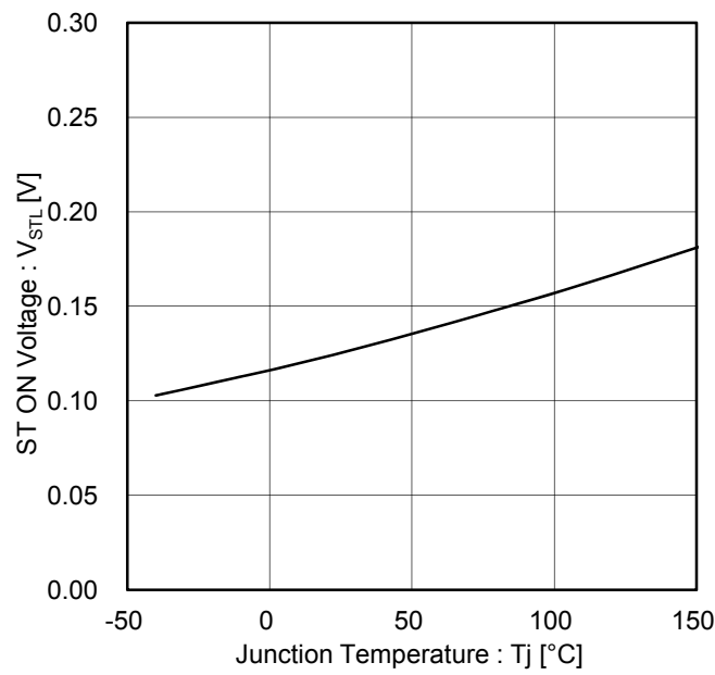
Figure 21. ST ON Voltage vs. Temperature
