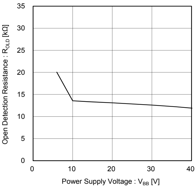
Figure 25. Open Detection Resistance vs. Power Supply Voltage
