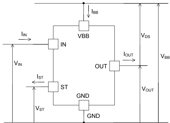
Figure 3. Voltage/Current Definition
