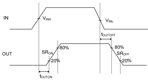
Figure 36. Slew Rate
