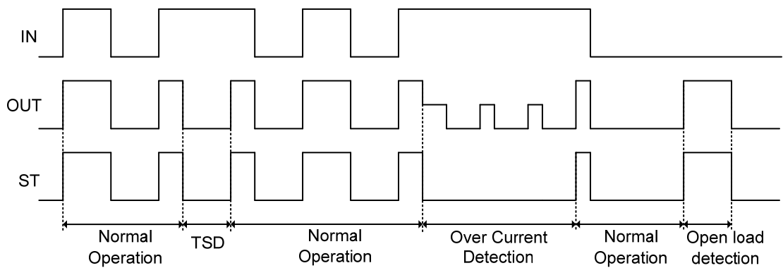
Figure 38. Timing Chart
