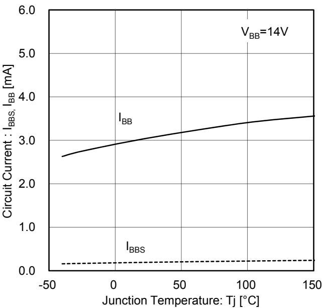
Figure 9. Circuit Current vs. Temperature
