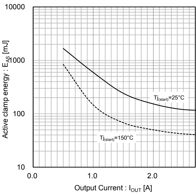
Figure 27. Active Clamp Energy vs. Output Current
