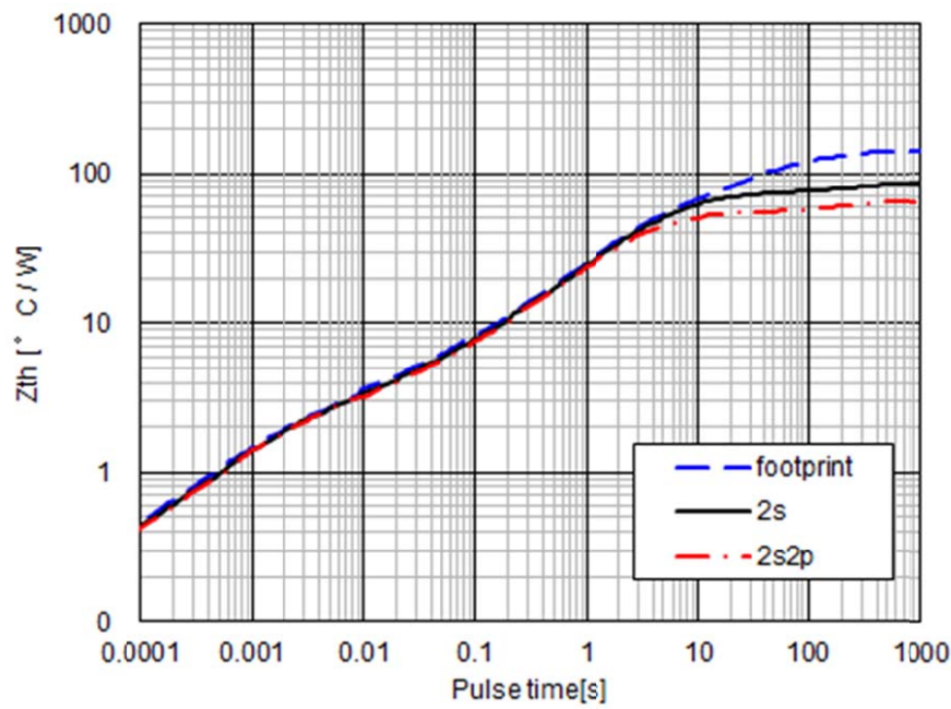
Figure 7. Thermal Resistance
