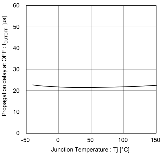
Figure 19. Propagation Delay at OFF vs. Temperature
