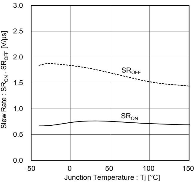
Figure 17. Slew Rate vs. Temperature
