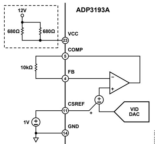
Figure 6. Positioning Voltage
