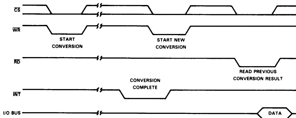
FIGURE 5. MODE 1 — STARTING NEW CONVERSION BEFORE READING PREVIOUS RESULT
