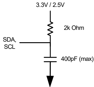
Figure 6: AC Output Test Load (I²C)
