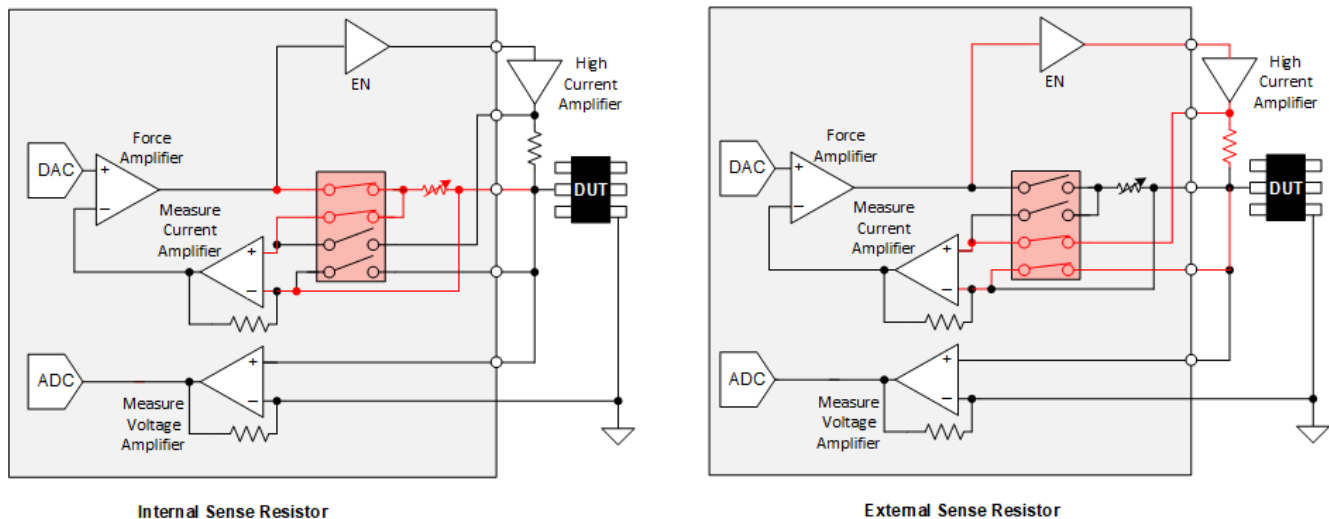
Figure 10-1. High Current Range Selection Using External Resistor
