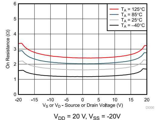
Figure 7-6. On-Resistance vs Temperature
