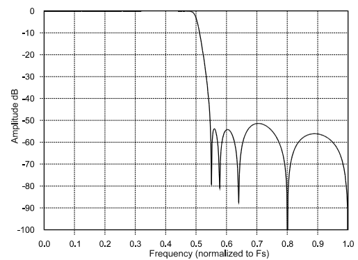
Figure 31. DAC Stopband
