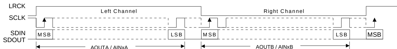
Figure 17. Left-Justified Format
