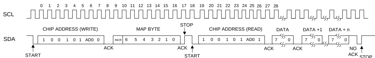
Figure 21. Control Port Timing, I²C Read
