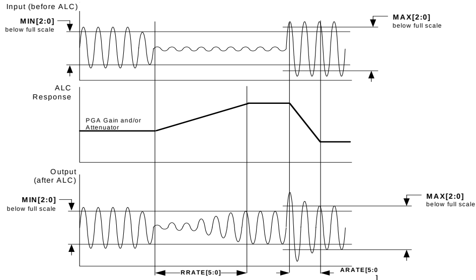
Figure 8. ALC
