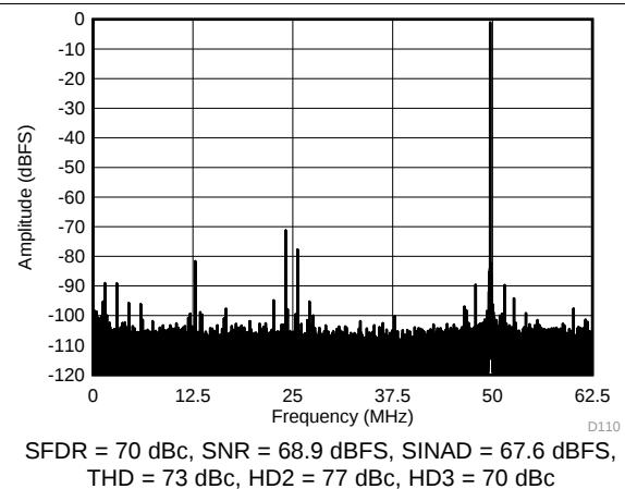
Figure 103. FFT for 450-MHz Input Signal (Dither Off)
