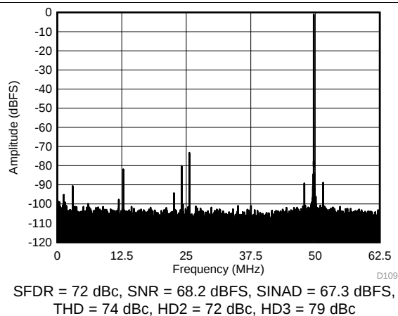
Figure 102. FFT for 450-MHz Input Signal (Dither On)
