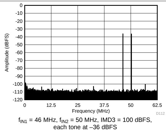
Figure 105. FFT for Two-Tone Input Signal ( -36\text{ dBFS} at 46 MHz and 50 MHz)
