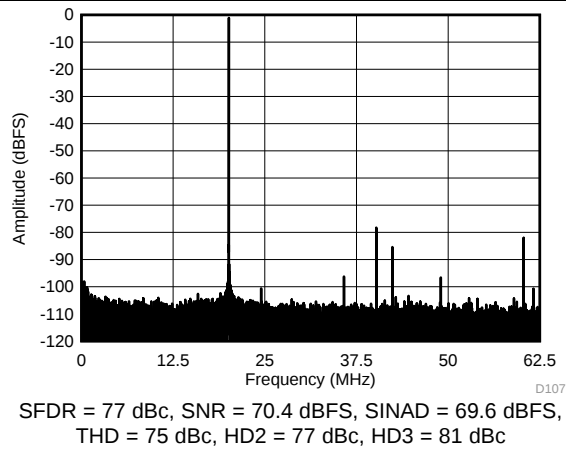
Figure 100. FFT for 270-MHz Input Signal (Dither On)
