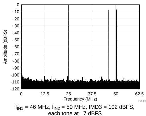
Figure 104. FFT for Two-Tone Input Signal ( -7\text{ dBFS} at 46 MHz and 50 MHz)
