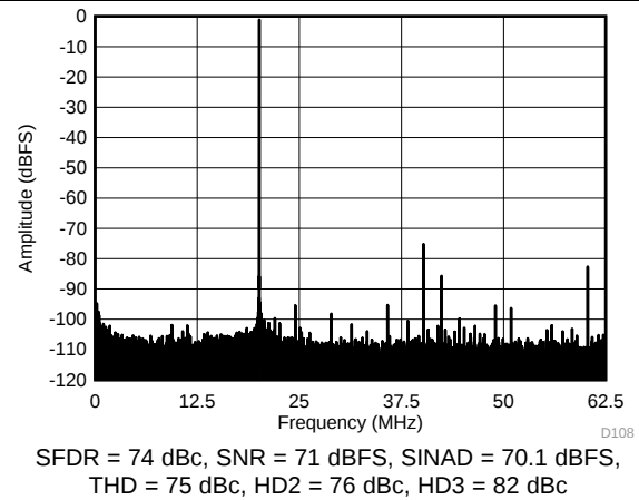
Figure 101. FFT for 270-MHz Input Signal (Dither Off)
