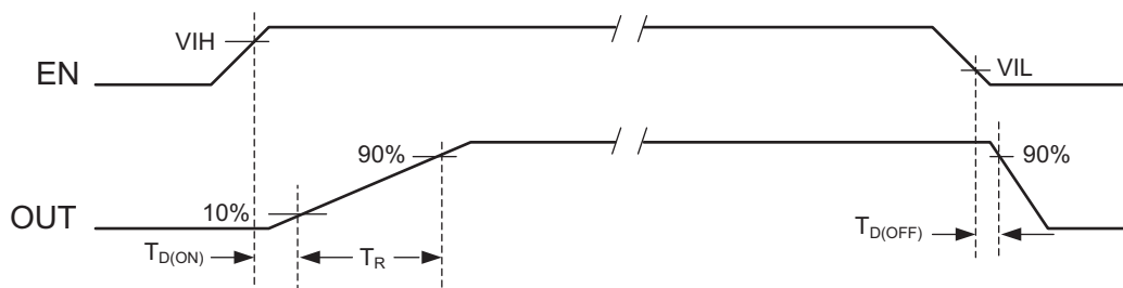
Figure 1. AOZ1361DI Timing
