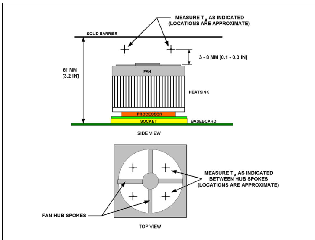
Figure 3-2. Locations for Measuring Local Ambient Temperature, Active ATX Heatsink
