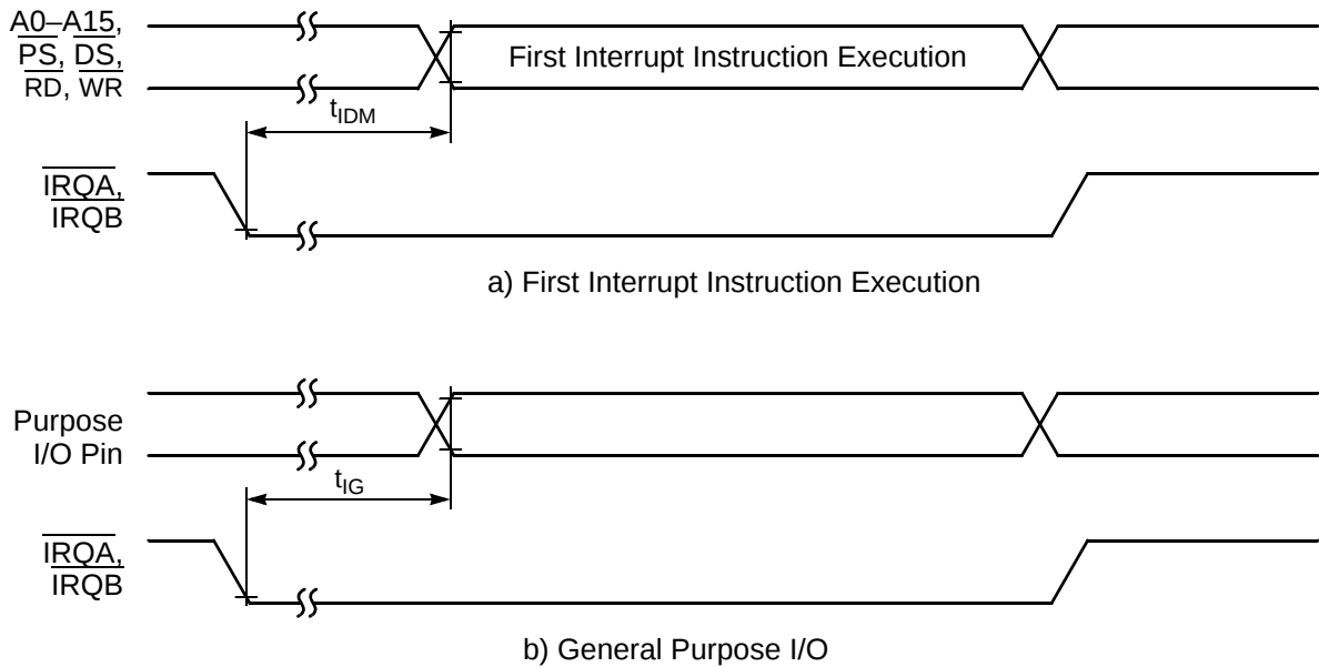
Figure 3-14 External Level-Sensitive Interrupt Timing
