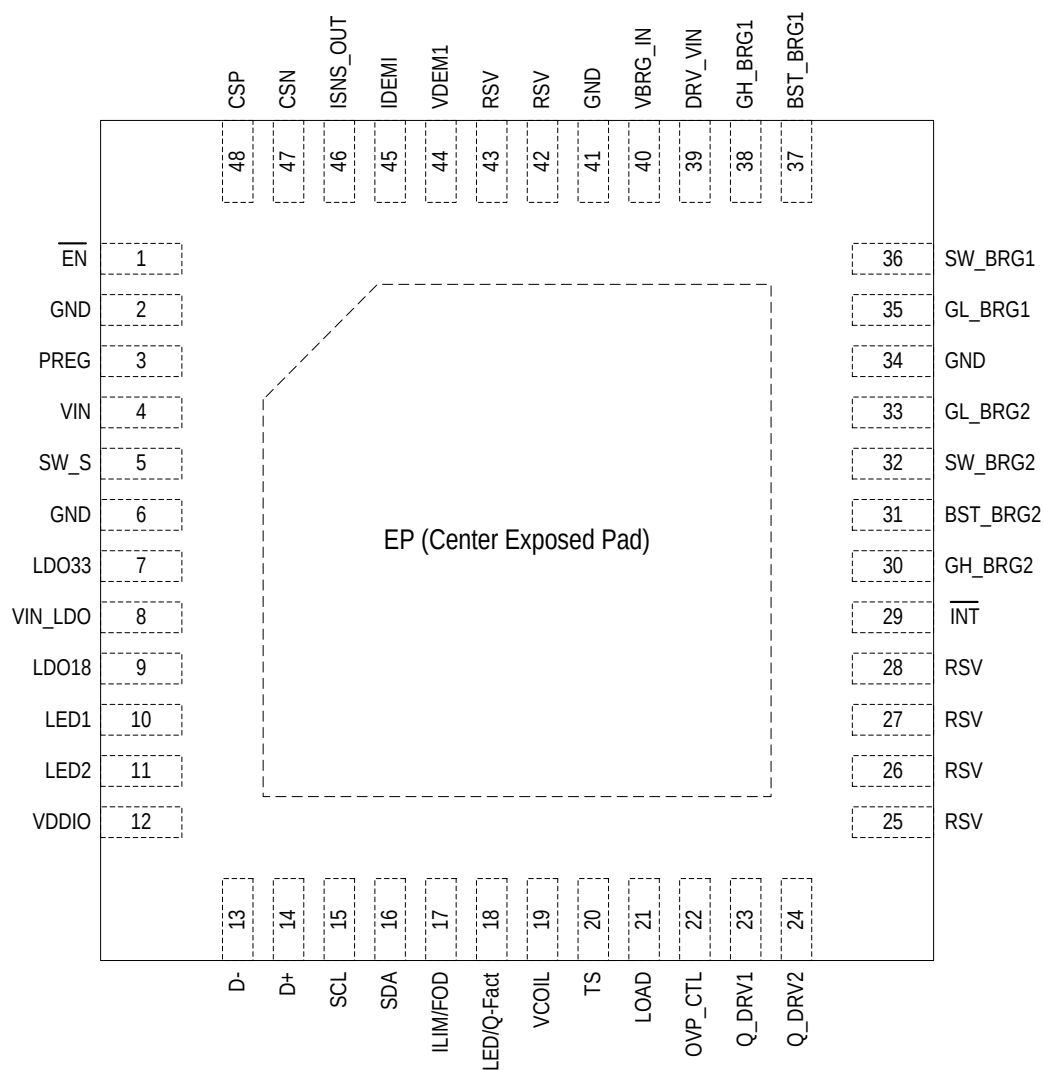
Figure 1. Pin Assignments
