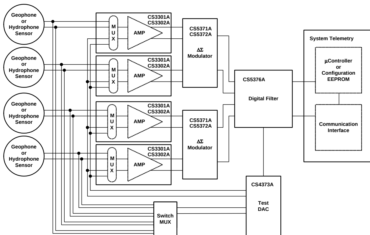
Figure 3. Multi-Channel System Architecture
