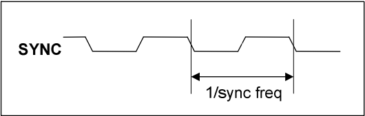
Figure 6 System Clock Timing Requirements
