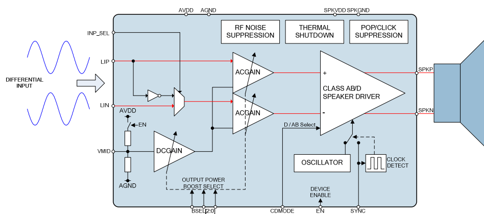
Figure 4 Differential Mode Audio Signal Paths
