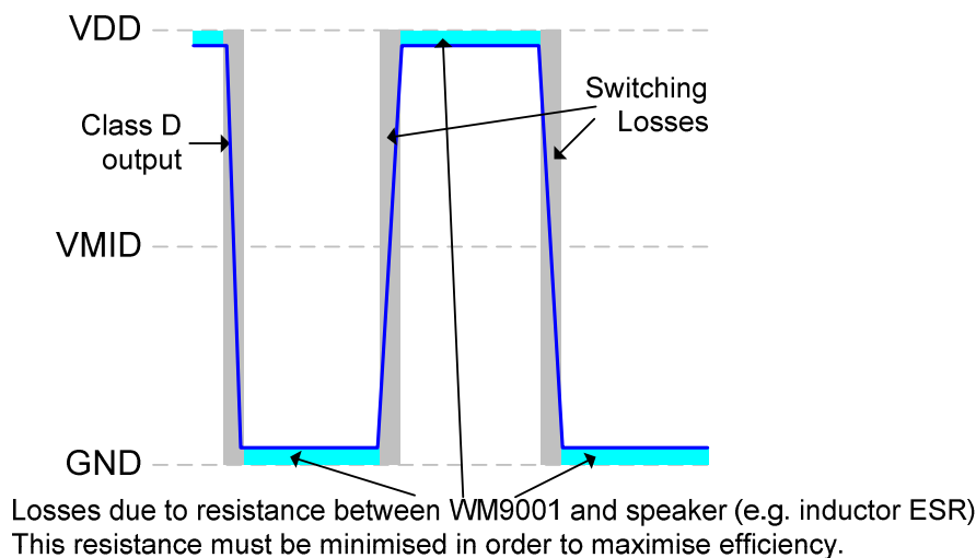
Figure 12 Speaker Connection Losses
