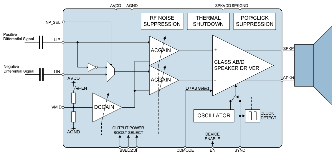
Figure 8 Operation of WM9001 as Stand-alone Differential Amplifier
