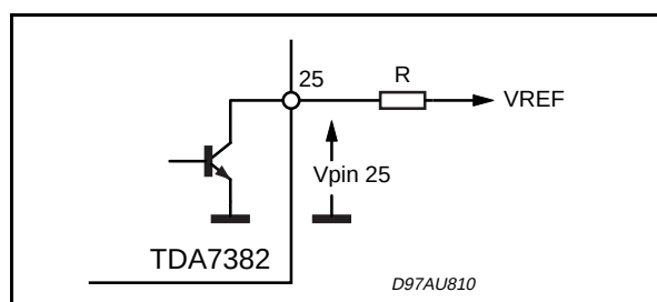
Figure 12: Diagnostics circuit.
