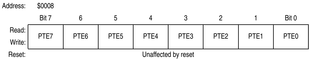
Figure 10-13. Port E Data Register (PTE)
